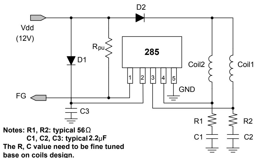
12V DC Brush-less Fan with FG output function
