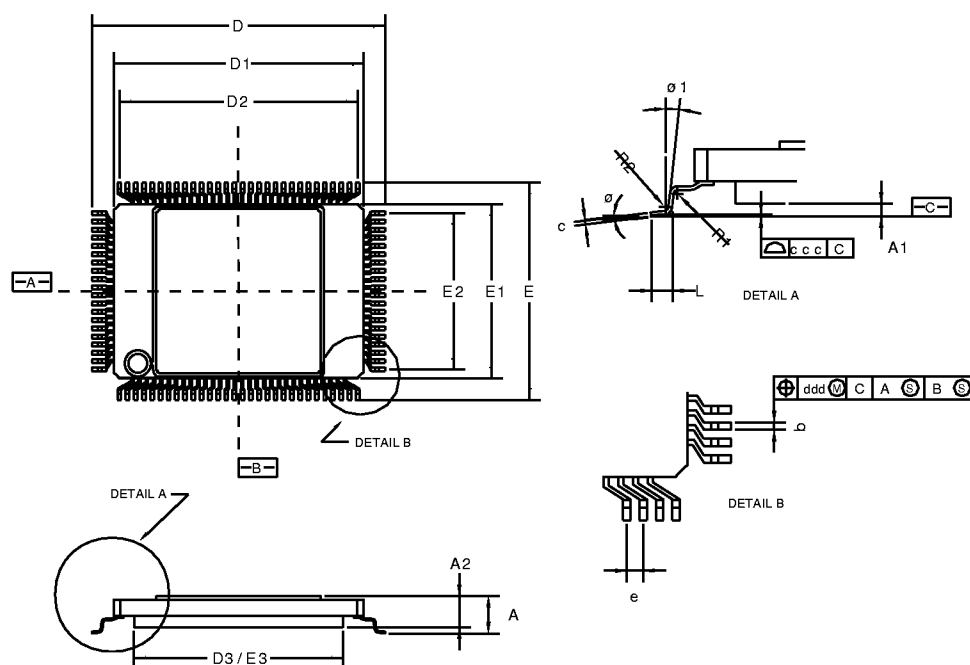
100-LEAD QUAD FLATPACK - GC100
