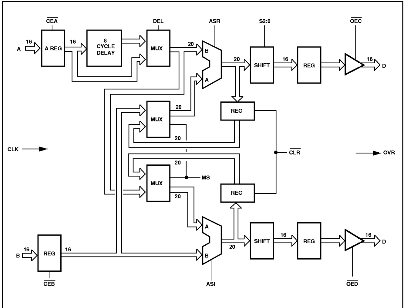
Fig. 3 Block diagram
