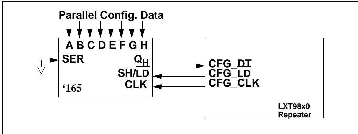
Figure 17 Serial Configuration Interface
