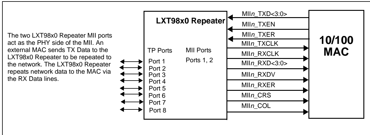
Figure 10 LXT9880 Repeater MII Operation
