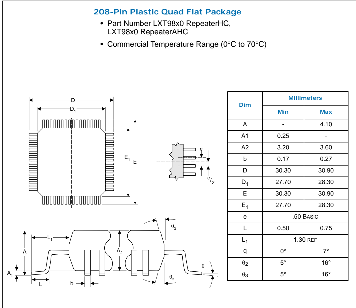
Figure 42 Package Specifications for Commercial Temperature
