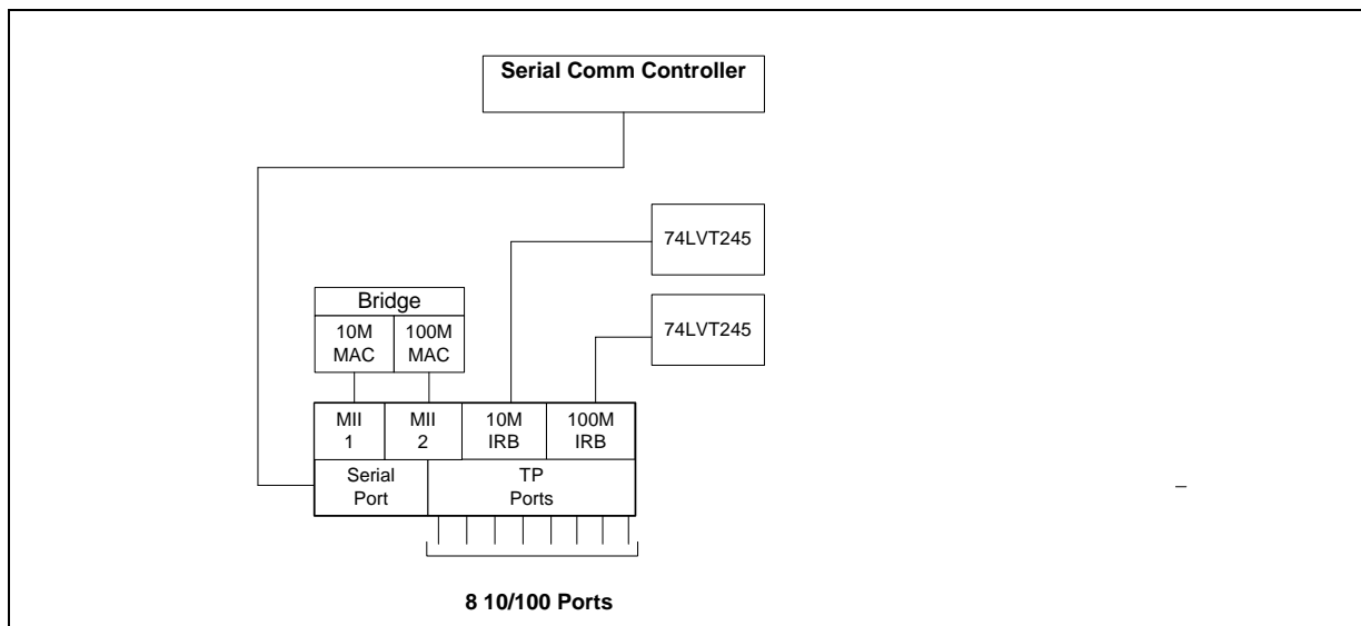
Figure 19 8-Port Managed 10/100 Stackable Repeater
