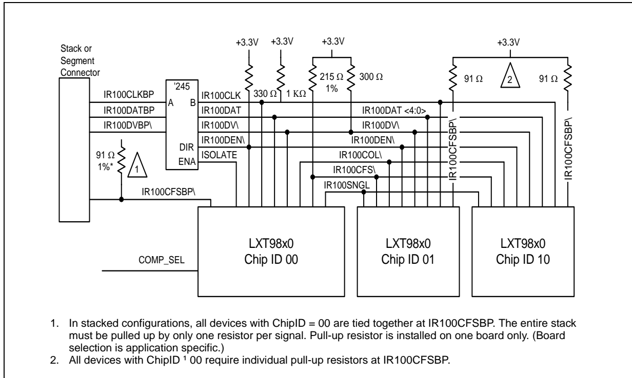
Figure 30 Typical 100 Mbps IRB Implementation
