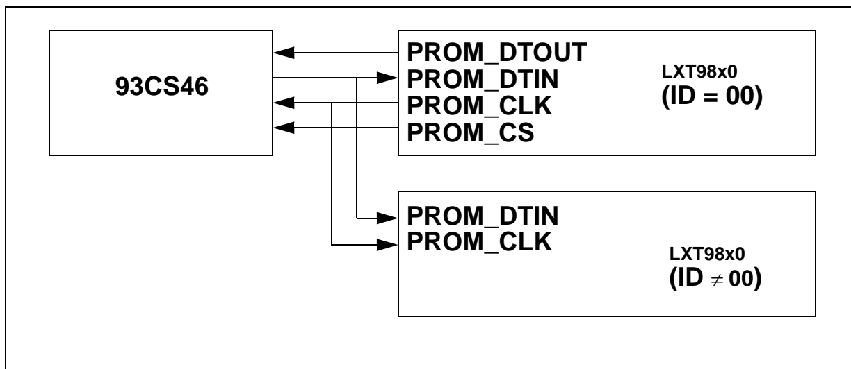
Figure 25 Serial PROM Interface
