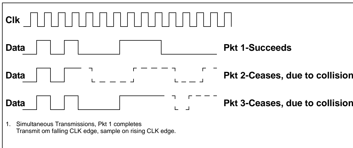
Figure 12 SMI Collision Handling
