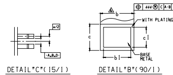
DETAIL "C" (15/1)
