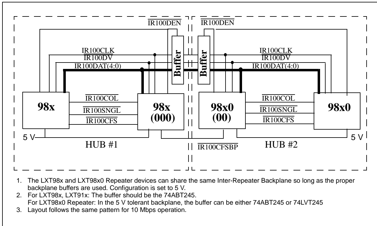
Figure 29 100 Mbps Backplane Connection between LXT98x and LXT98x0 Repeater
