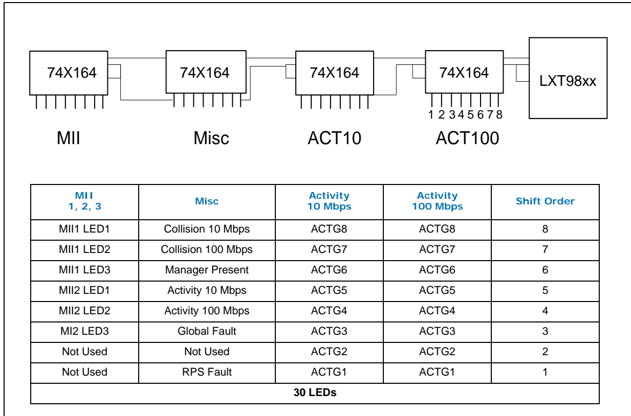
Figure 6 Serial LED Shift Loading
