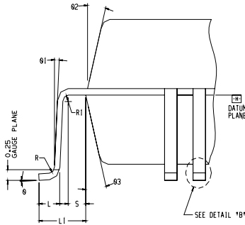
DETAIL "A" (20/1)
