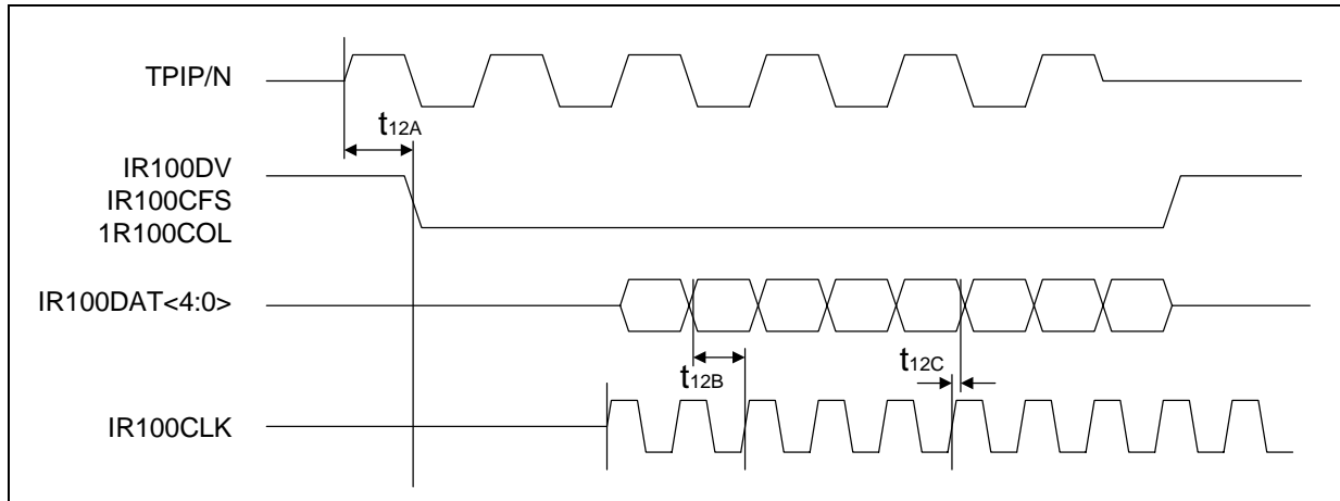
Figure 37 100 Mbps TP-to-IRB Timing
