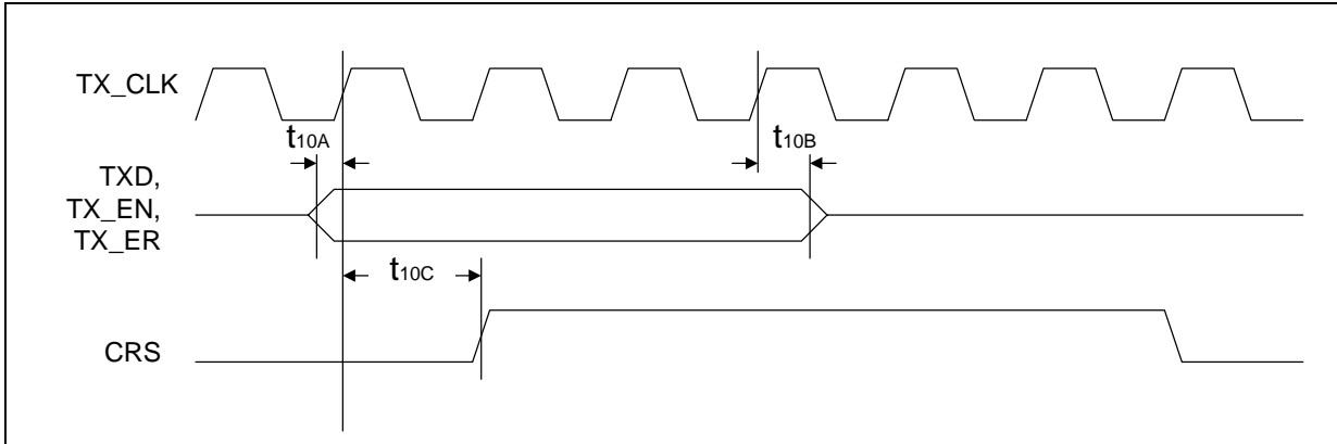
Figure 35 10BASE-T MII-to-TP Timing
