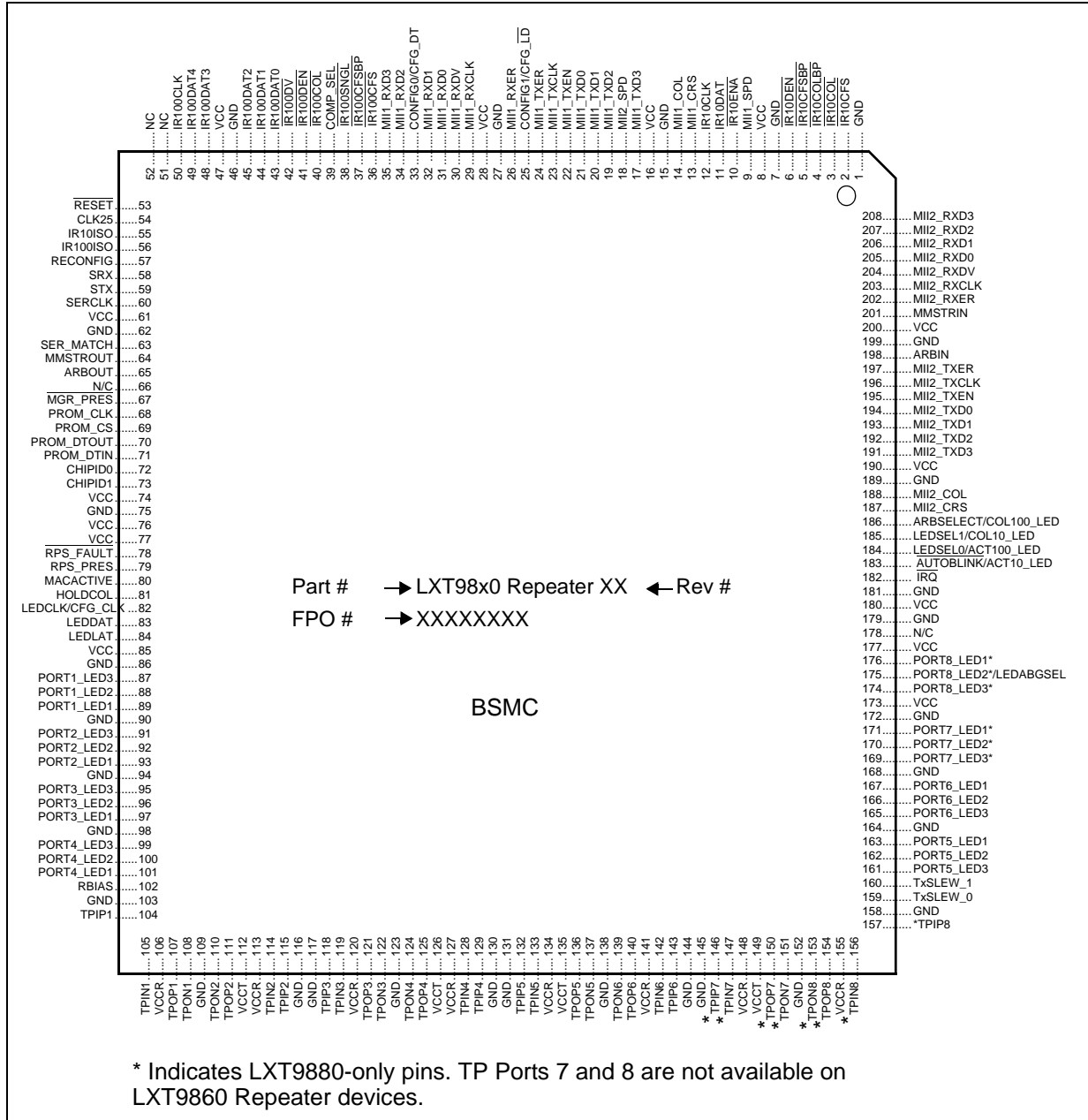
Figure 2 Pin Assignments
