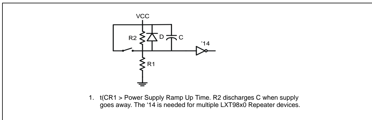
Figure 26 Typical Reset Circuit
