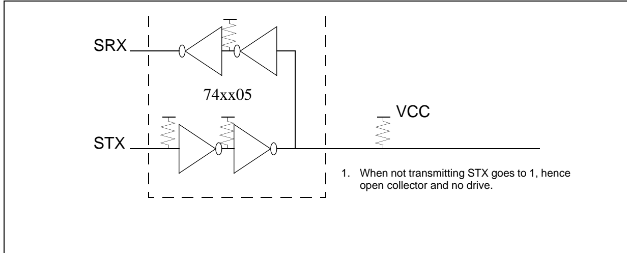
Figure 23 Typical Serial Management Interface Connections
