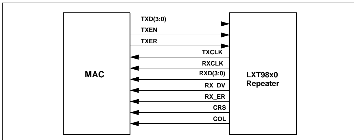
Figure 4 MII Interface
