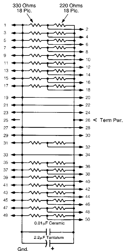
50-Position, Single-Ended Part No. 869587-1
