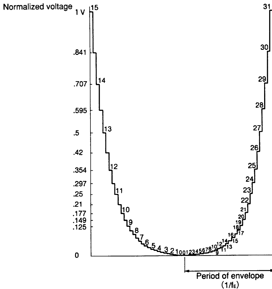
Fig.1 Output level of D/A convertor
