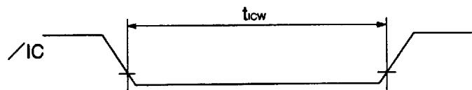
(2) Reset timing
