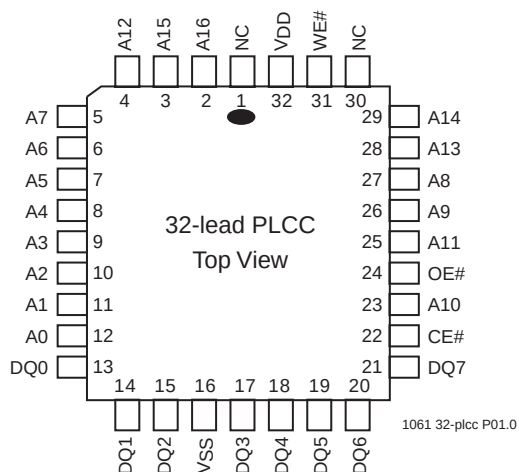
FIGURE 1: PIN ASSIGNMENTS FOR 32-LEAD PLCC
