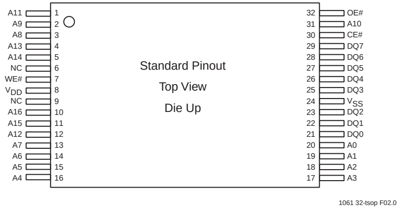
FIGURE 2: PIN ASSIGNMENTS FOR 32-LEAD TSOP
