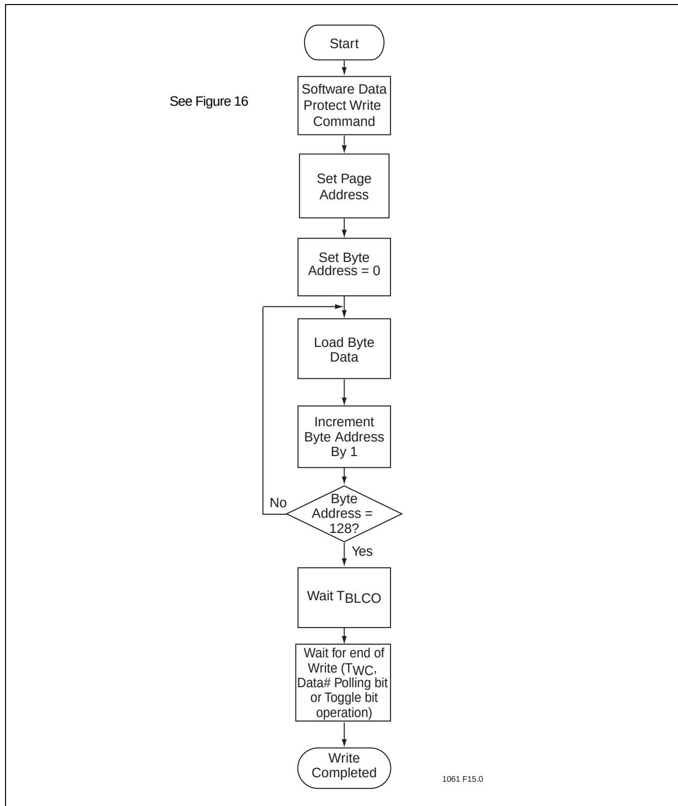
FIGURE 14: WRITE ALGORITHM
