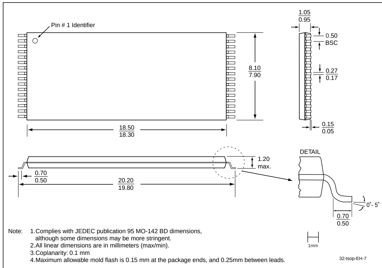
32-LEAD THIN SMALL OUTLINE PACKAGE (TSOP) 8MM X 20MM SST PACKAGE CODE: EH
