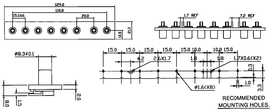
RIGHT ANGLE PCB MOUNT JACK
