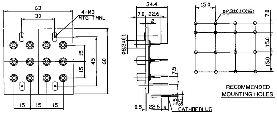
STRAIGHT PCB MOUNT JACK
