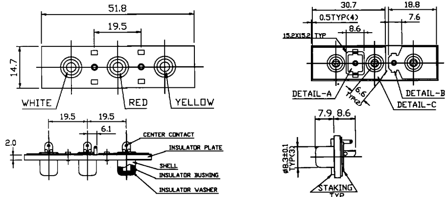
STRAIGHT CHASSIS SCREW JACK
