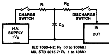
FIGURE 1. ELECTROSTATIC DISCHARGE TEST
