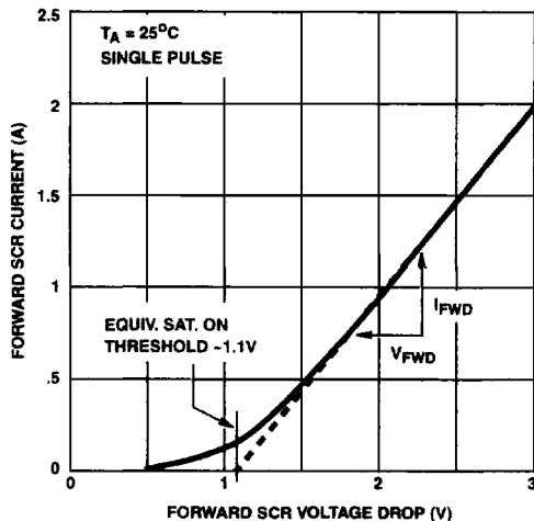
FIGURE 5. HIGH CURRENT SCR FORWARD VOLTAGE DROP CURVE
