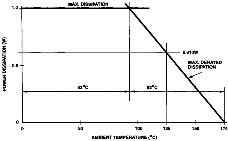
FIGURE 7. SP720MD DERATING CURVE FOR THE 82°C/W THERMAL RESISTANCE OF THE SIDEBRAZE 16 LEAD CERAMIC PACKAGE, DERATED 12.2mW/°C FROM A MAXIMUM P D OF 1.0W AT 93°C
