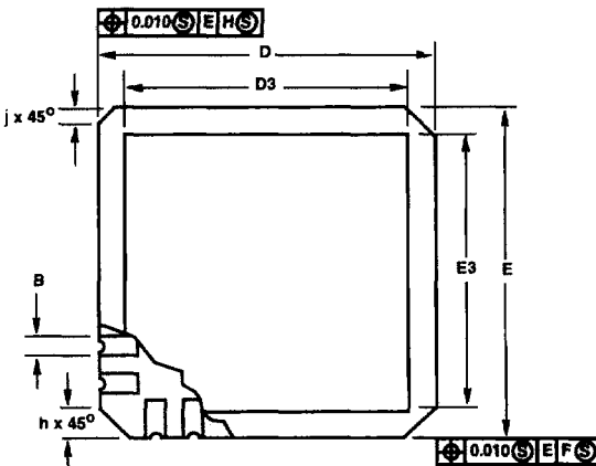
J20.A MIL-STD-1835 CQCC1-N20 (C-2) 20 PAD CERAMIC LEADLESS CHIP CARRIER PACKAGE
