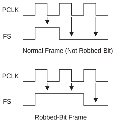
Figure 25. Robbed-Bit Frame
