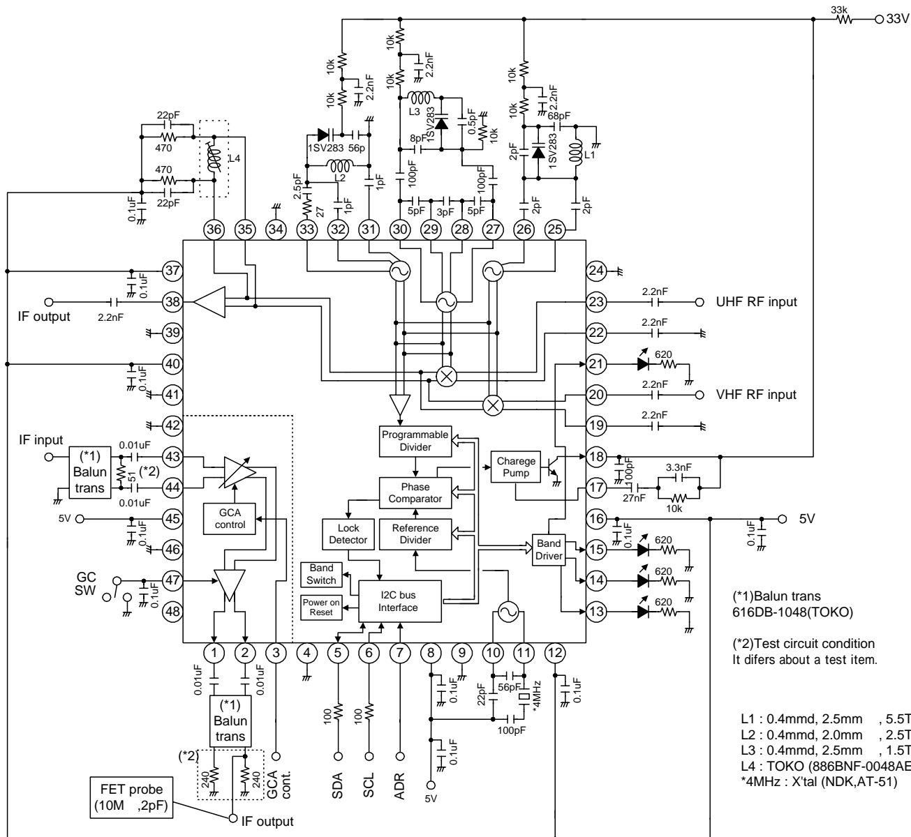
Figure.4 Test Circuit 3
