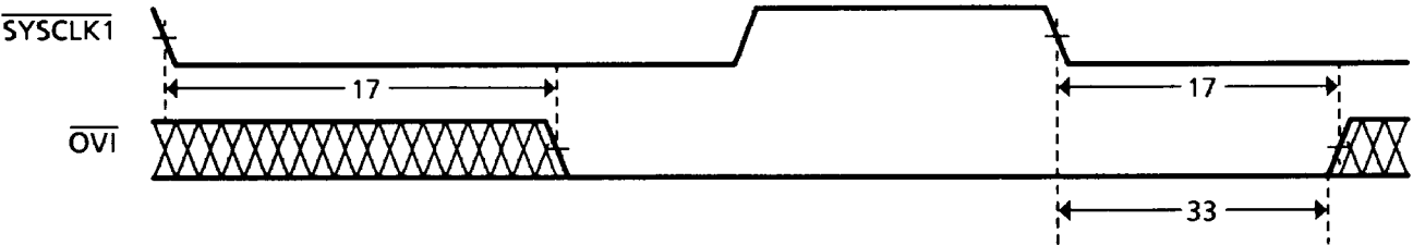
Figure 18. Fixed-Point Overflow Timing
