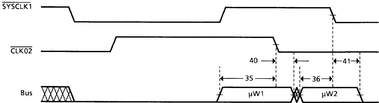
Figure 9. Microcode Bus Timing
