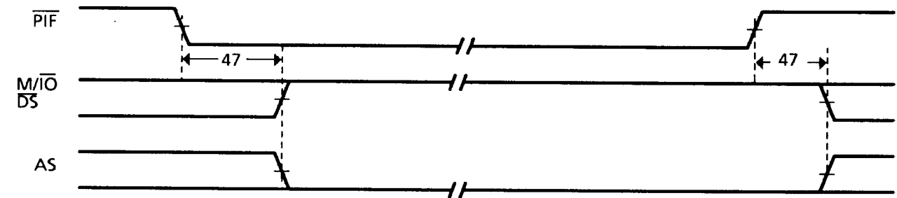
Figure 19. Instruction Abort Fault Timing
