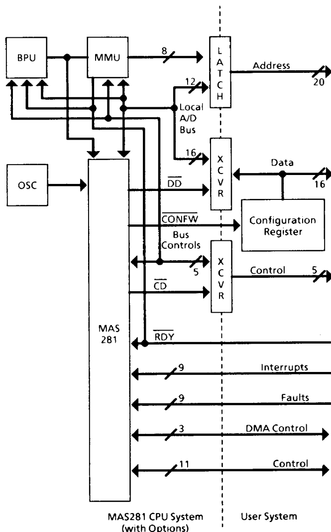
Figure 4. Typical MAS281/MA17504 System Interface
