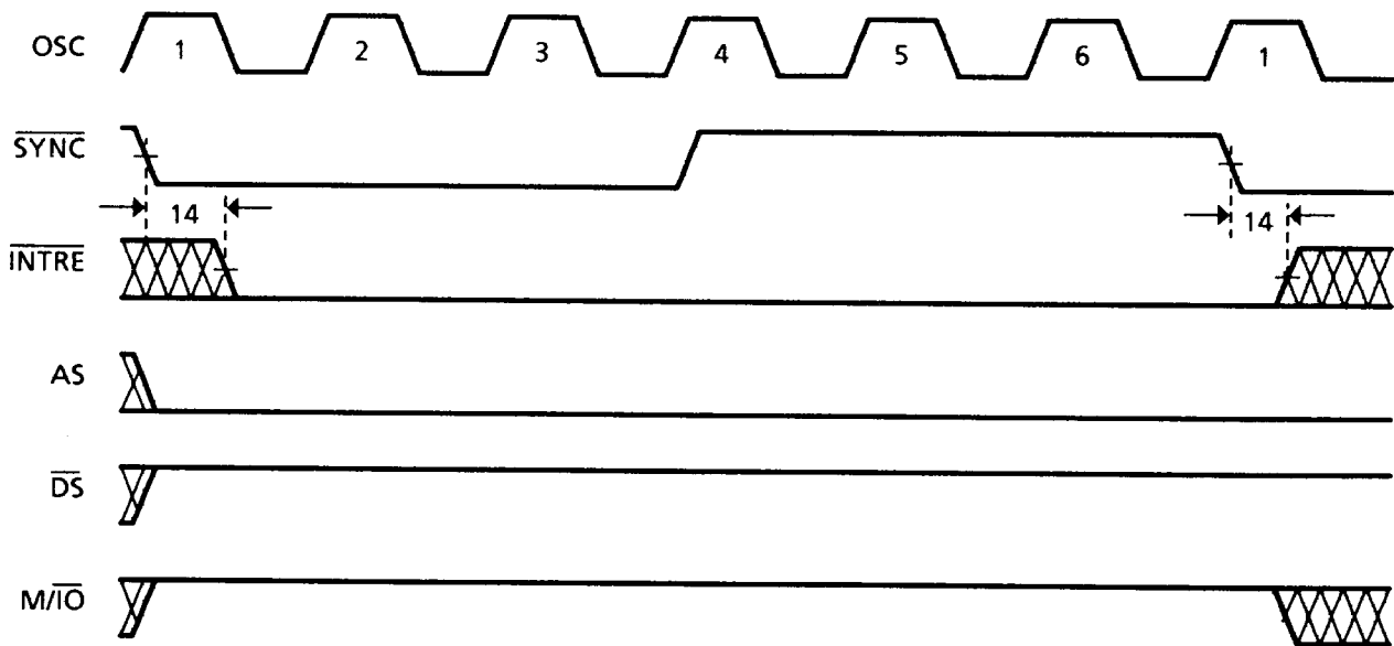
Figure 20. Interrupt Unit Microcode Enable Timing
