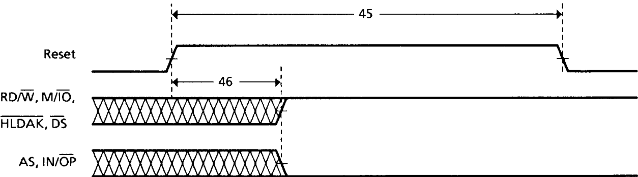
Figure 6. Reset Timing
