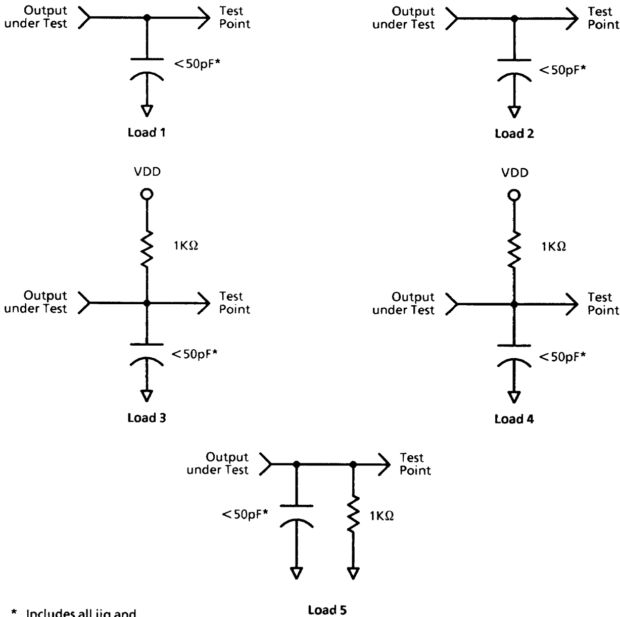
Figure 5. Test Loads
