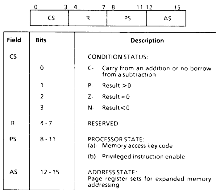
Figure 3. Status Word Format
