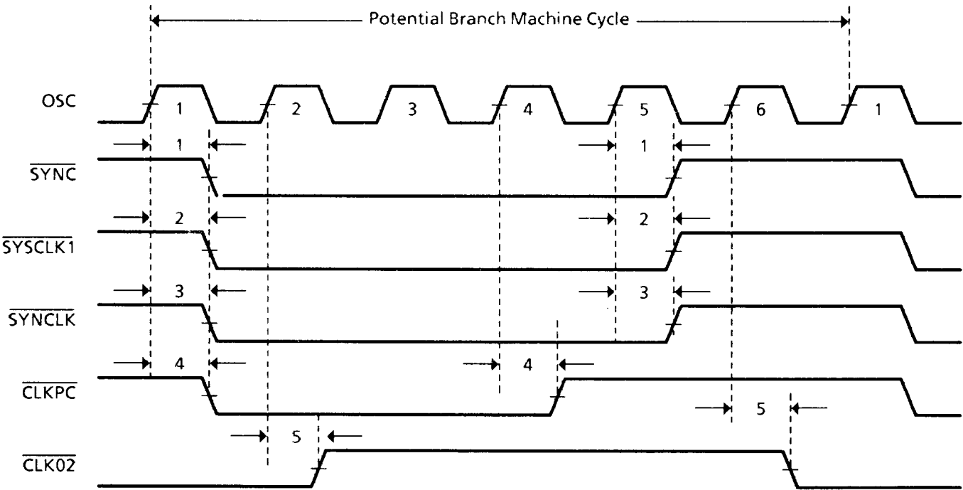
Figure 8. Potential Branch Clock Timing
