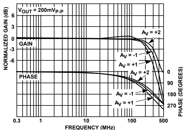
FIGURE 10. FREQUENCY RESPONSE
