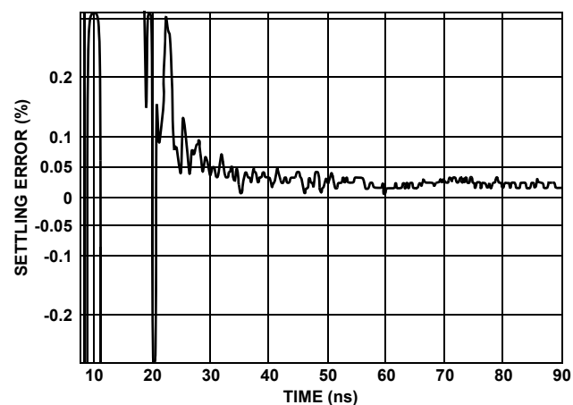
FIGURE 33. SETTLING RESPONSE
