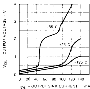
Output Low Voltage Versus Output Current
