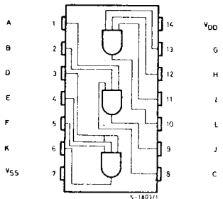
For 4073B
