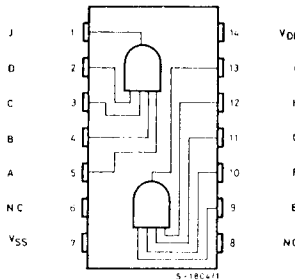
For 4082B
