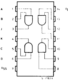
For 4081B
