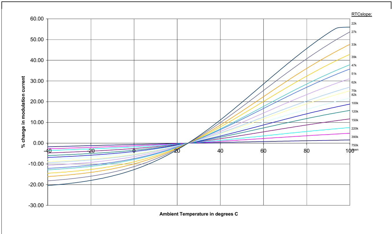
Figure 3-2. Selecting TC SLOPE Resistance in Common Anode Configuration
