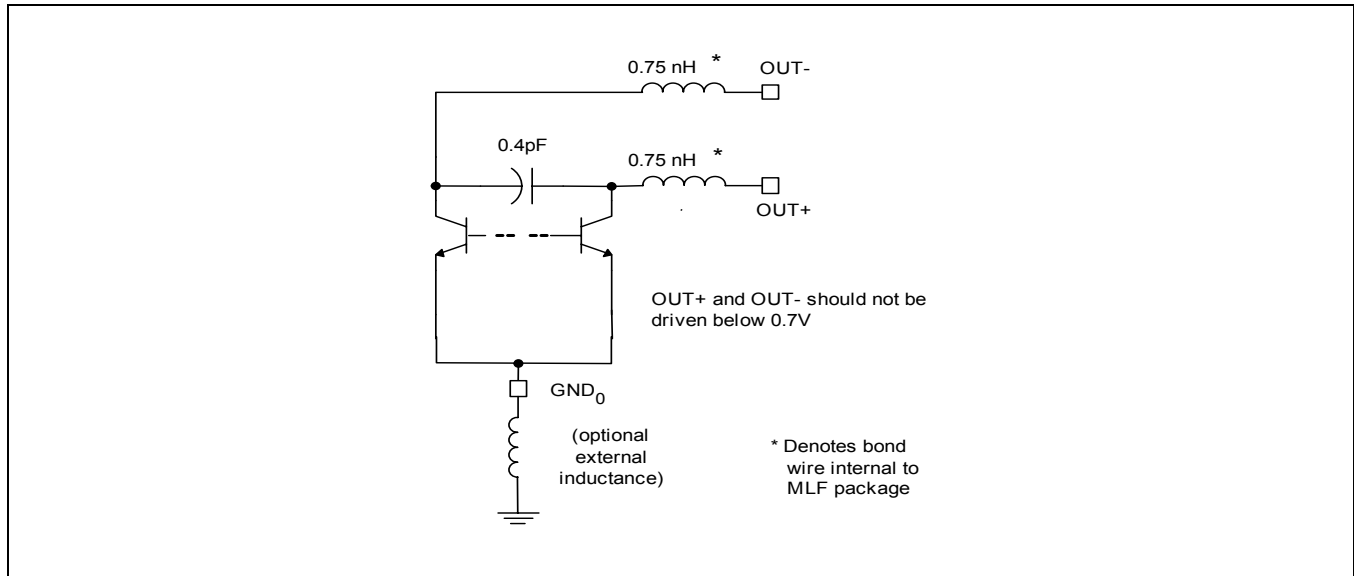
Figure 3-4. Modulator Output
