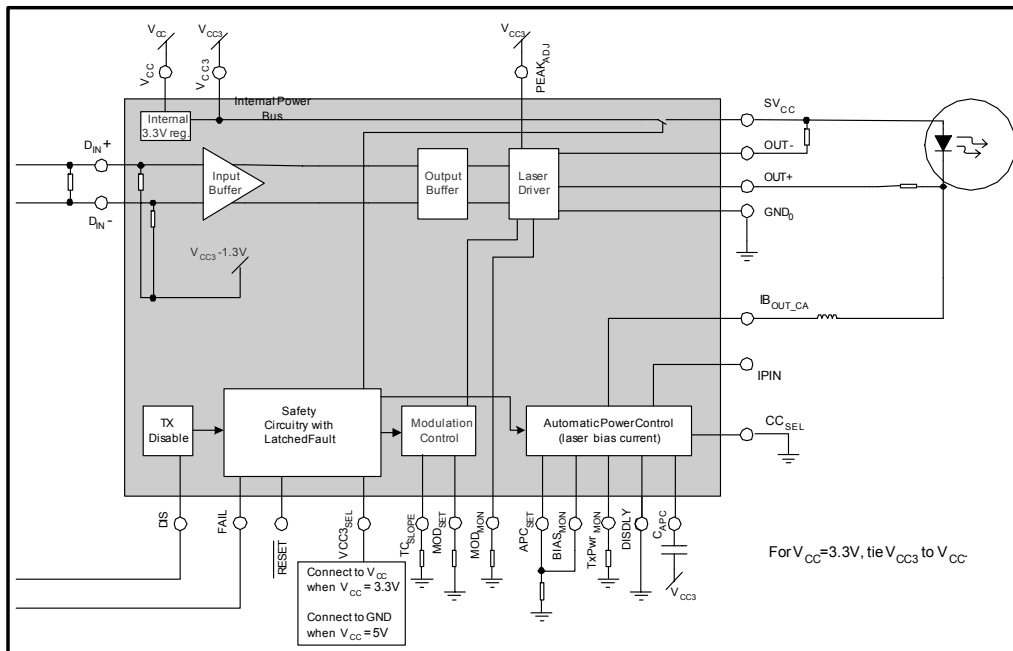
Figure 3-6. Video Application Block Diagram
