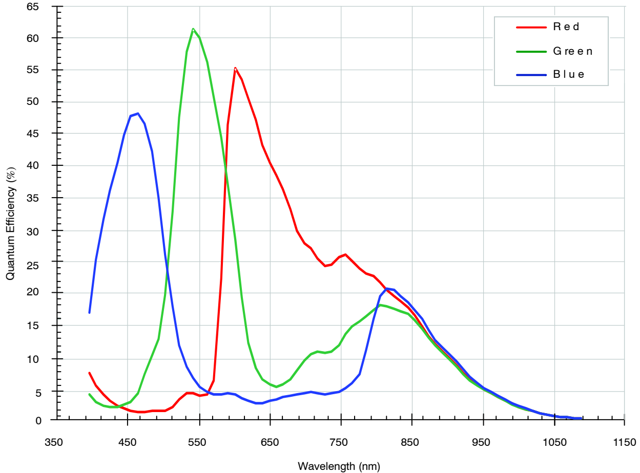
Figure 43. Quantum Efficiency
