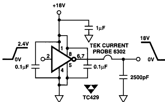
Figure 3. Peak Output Current Test Circuit
