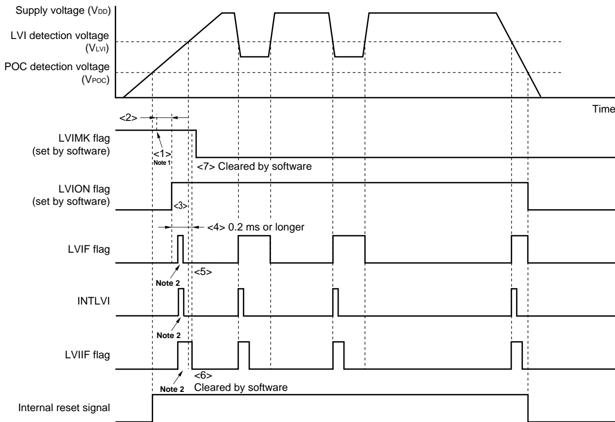
Figure 16-5. Timing of Low-Voltage Detector Interrupt Signal Generation
