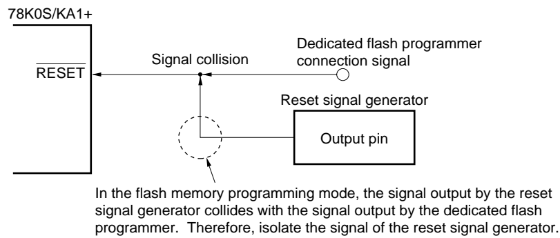
Figure 18-8. Signal Collision ( \overline{\text{RESET}} Pin)
