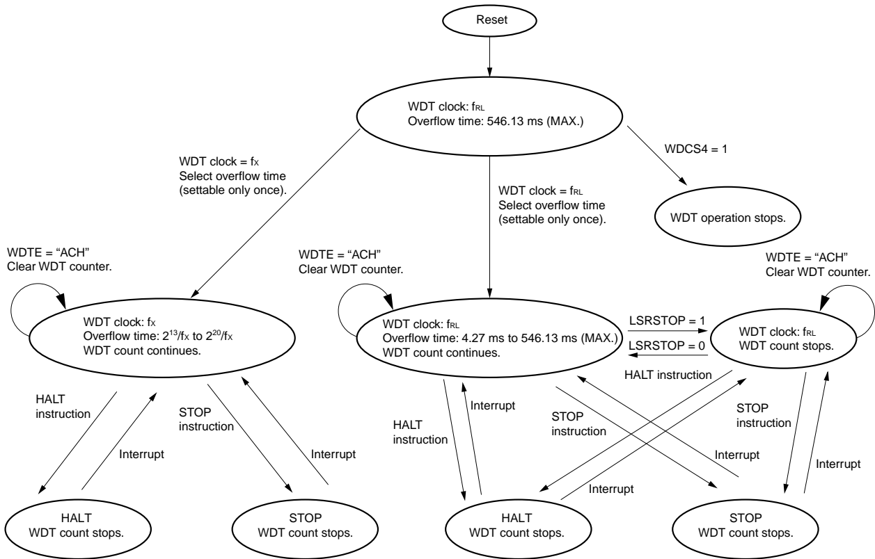
Figure 9-5. Status Transition Diagram When “Low-Speed Internal Oscillator Can Be Stopped by Software”
