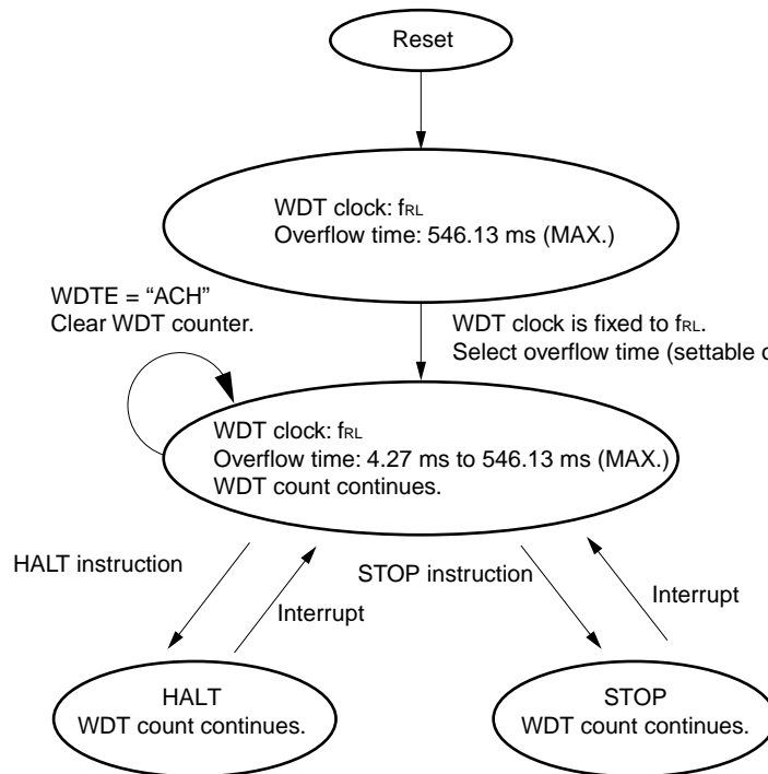
Figure 9-4. Status Transition Diagram When “Low-Speed Internal Oscillator Cannot Be Stopped” Is Selected by Option Byte
