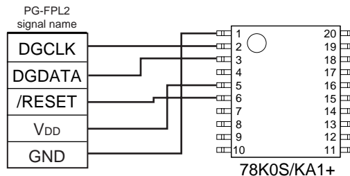
Figure 18-5. Wiring diagram with PG-FPL2
