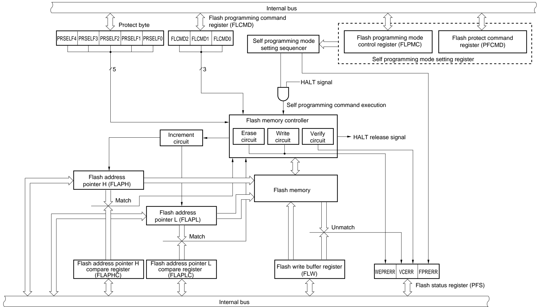
Figure 18-10. Block Diagram of Self Programming
