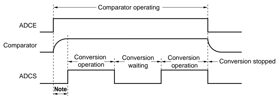
Figure 10-4. Timing Chart When Comparator Is Used
