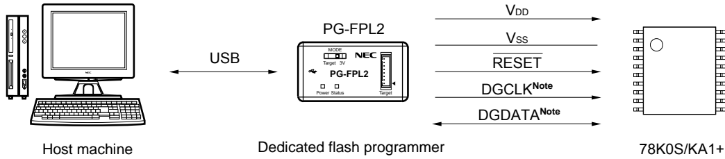
★ Figure 18-3. Environment for Writing Program to Flash Memory (PG-FPL2)
