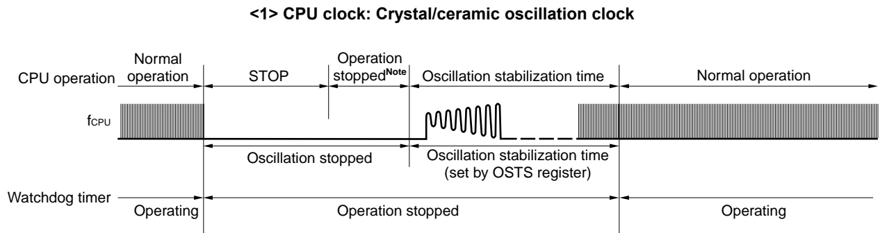
Figure 9-6. Operation in STOP Mode (WDT Operation Clock: Clock to Peripheral Hardware)
