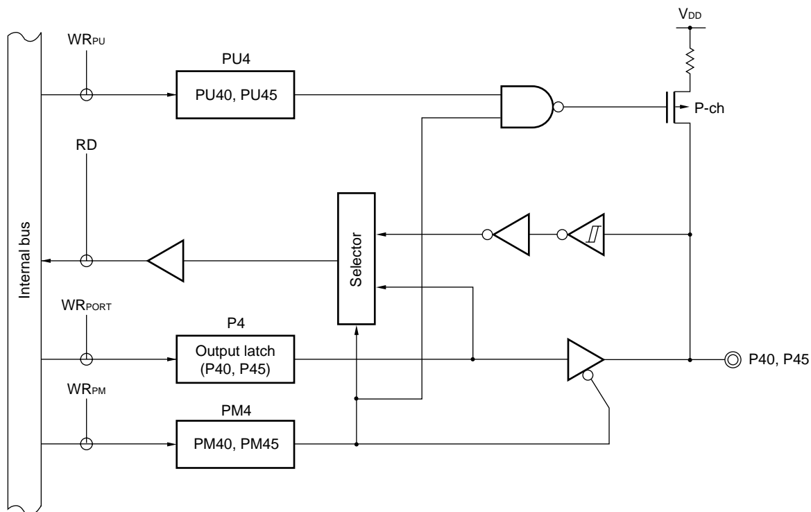
Figure 4-6. Block Diagram of P40 and P45
