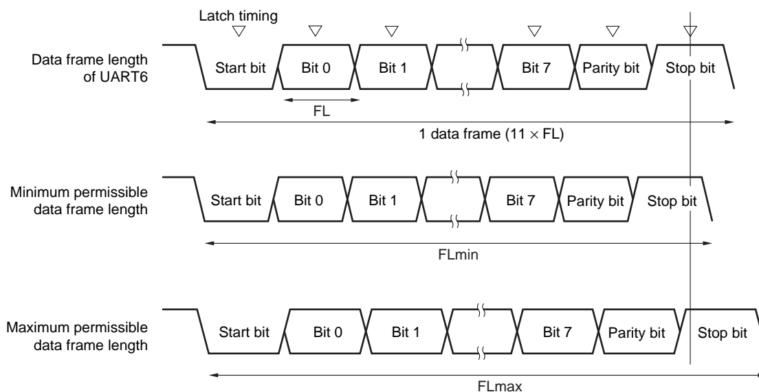
Figure 11-25. Permissible Baud Rate Range During Reception
