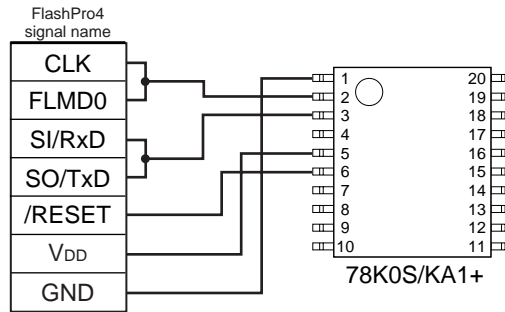
Figure 18-4. Wiring diagram with FlashPro4
