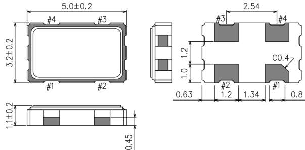
SG5032CAN
