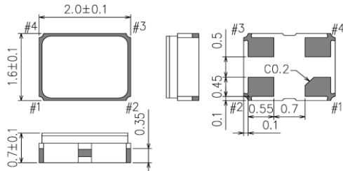
SG2016CAN
