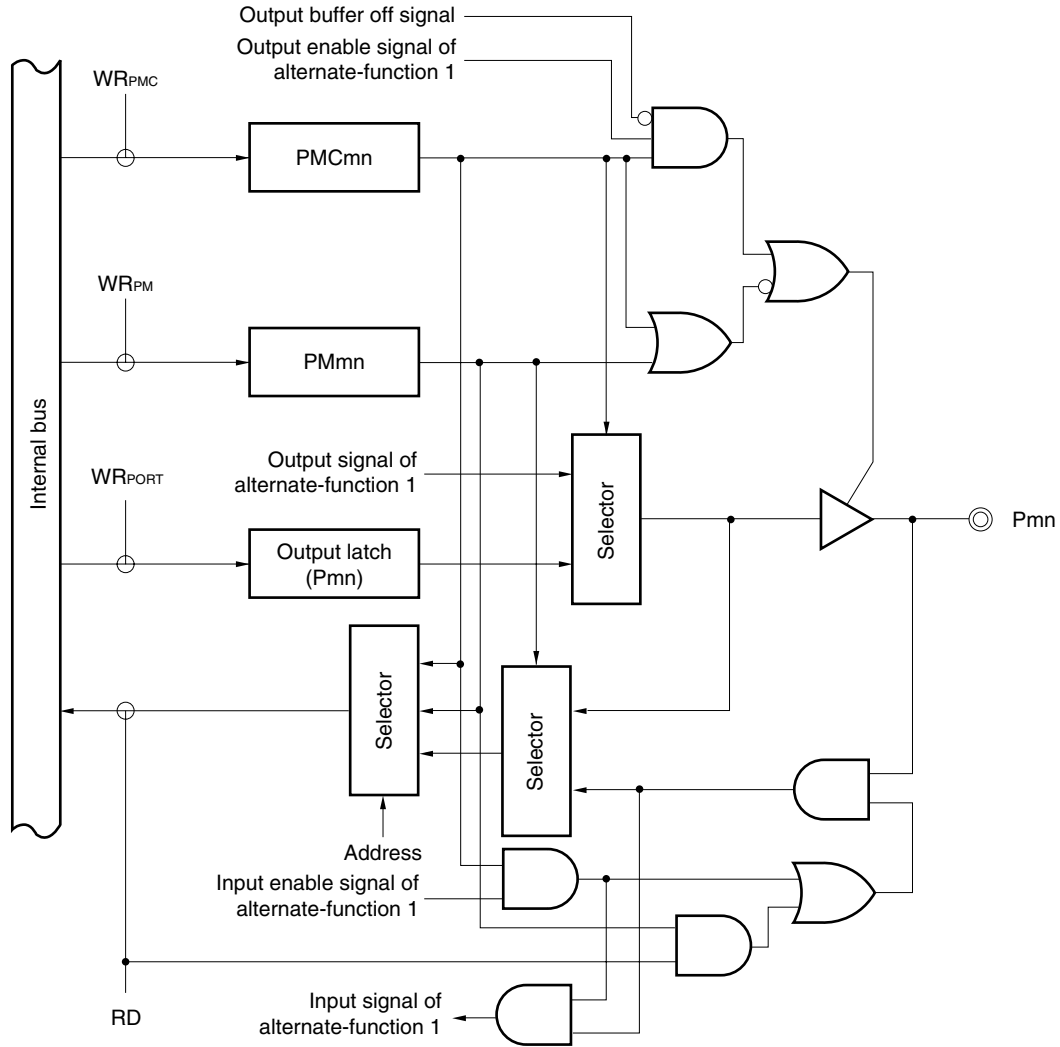
Figure 4-7. Block Diagram of Type C-4
