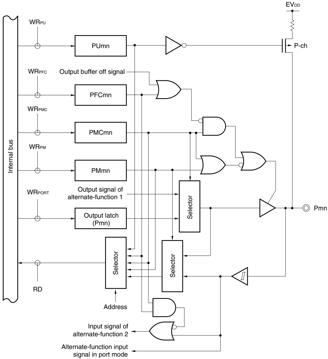
Figure 4-11. Block Diagram of Type E-1
