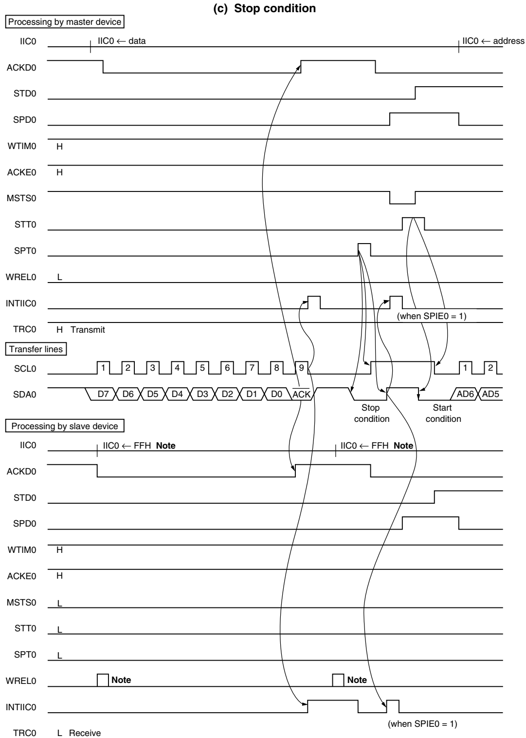
Figure 19-20. Example of Master to Slave Communication (When 9-Clock Wait Is Selected for Both Master and Slave) (3/3)
