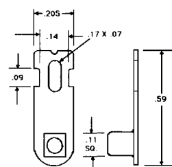
SOLDERING LUGS
