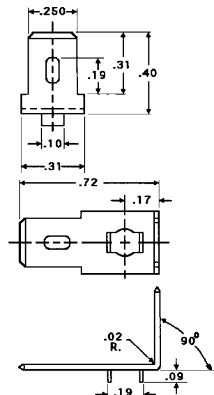
N4470 .032 BRASS QUICK DISCONNECT LUG
