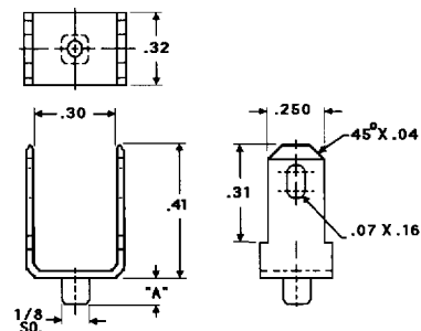
N4486 .032 BRASS QUICK DISCONNECT LUG
