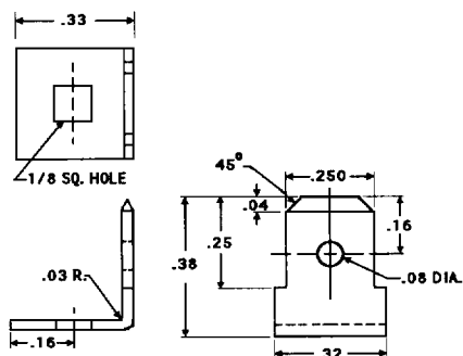
N4475 .032 BRASS QUICK DISCONNECT LUG
