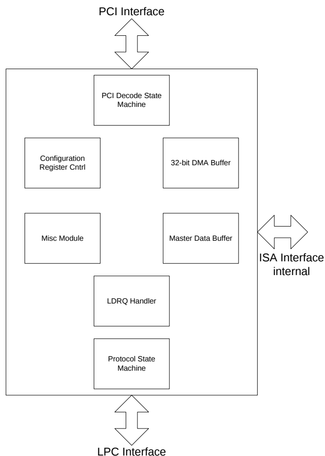
Figure 8-3: Block Diagram of LPC Module
