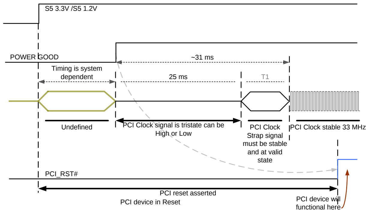
Figure 4-1: Straps Capture
