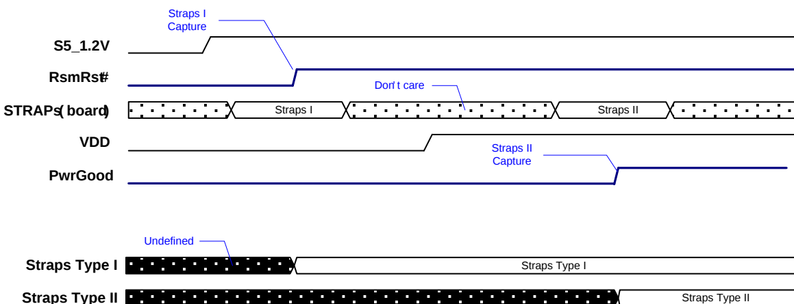
Figure 4-1: Straps Capture
