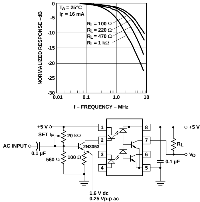
Figure 8. Frequency response.
