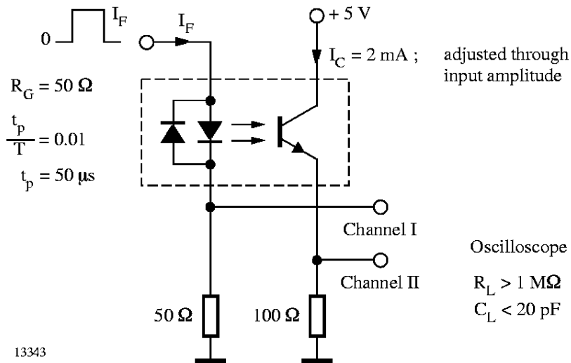
Figure 1. Test circuit
