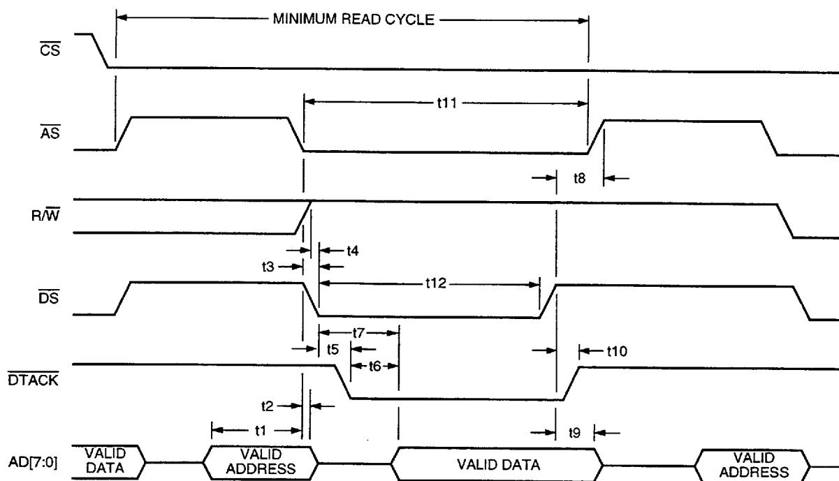
Figure 9. MODE 2—Read Cycle Timing (MPMODE = 0, MPMUX = 1)
