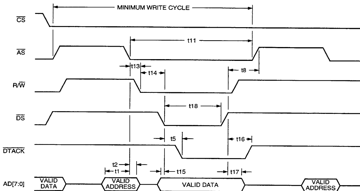
Figure 10. MODE 2—Write Cycle Timing (MPMODE = 0, MPMUX = 1)
