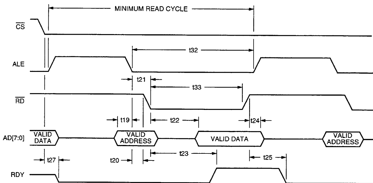
Figure 13. MODE 4—Read Cycle Timing (MPMODE = 1, MPMUX = 1)
