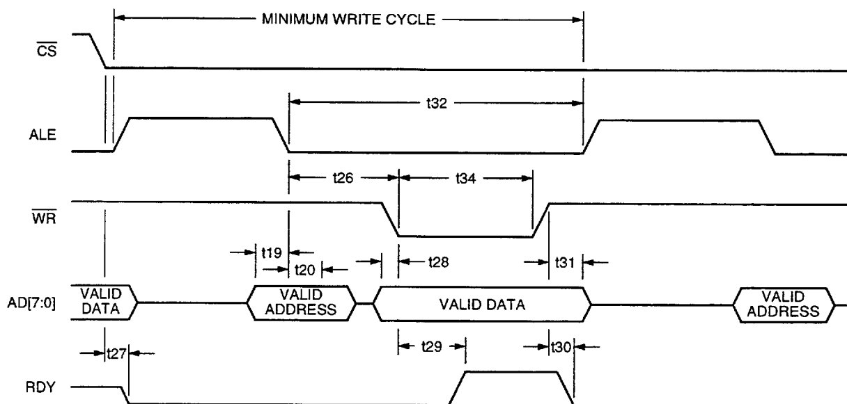
Figure 14. MODE 4—Write Cycle Timing (MPMODE = 1, MPMUX = 1)
