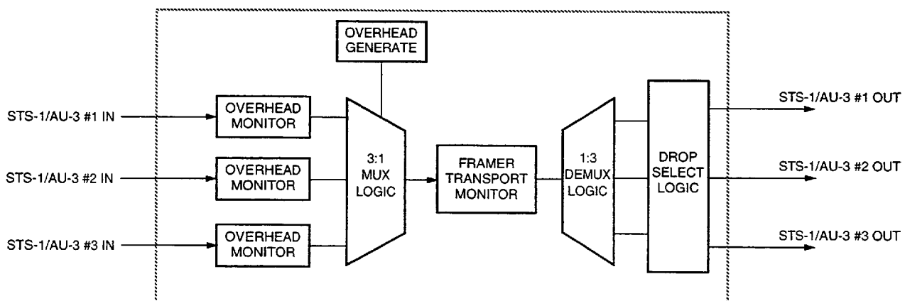
Figure 6. Digital Cross Connect
