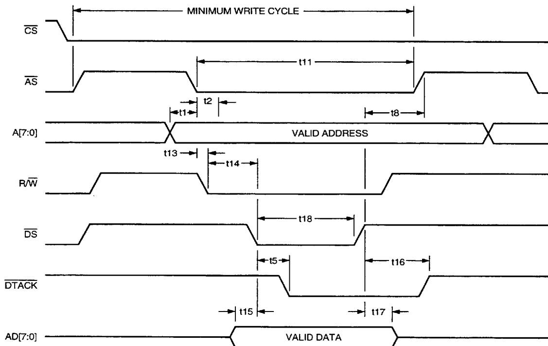
Figure 8. MODE 1—Write Cycle Timing (MPMODE = 0, MPMUX = 0)
