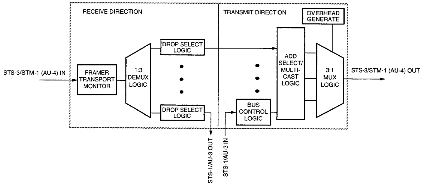
Figure 5. Add/Drop Multiplex
