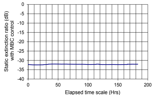
Stability with Time and Temperature
