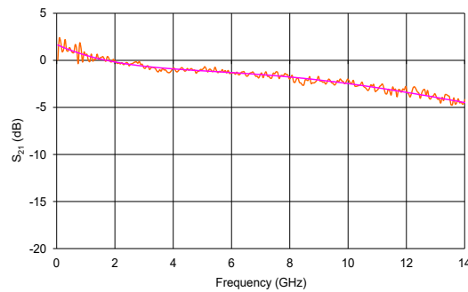
NIR-MX800-LN-20 Typical S_{21} Curve
