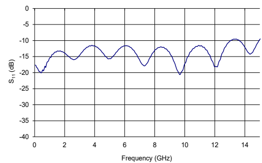
NIR-MX800-LN-10 Typical S_{11} Curve
