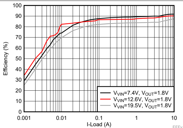
Figure 5. Efficiency Curve, V_{out}=1.8V
