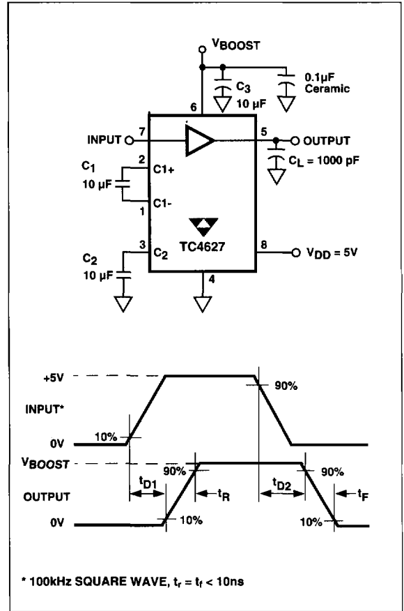
Figure 2. Non-Inverting Driver Switching Time
