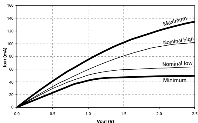
Figure 8: Normal Output Drive Curve Pull-Down Characteristics
