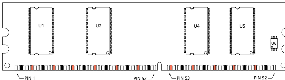
Figure 2: 184-Pin DIMM Pinouts
