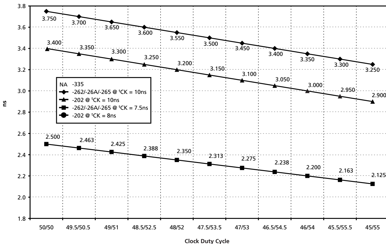
Figure 7: Derating Data Valid Window ( t_{QH} - t_{DQSQ} )
