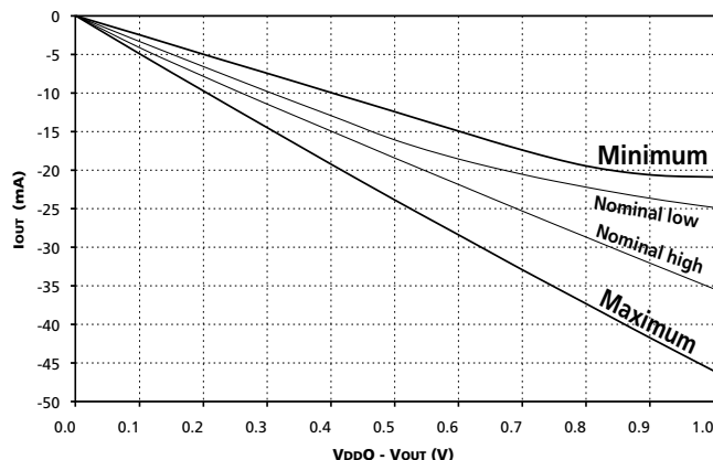
Figure 11: Reduced Output Drive Curve Pull-Up Characteristics
