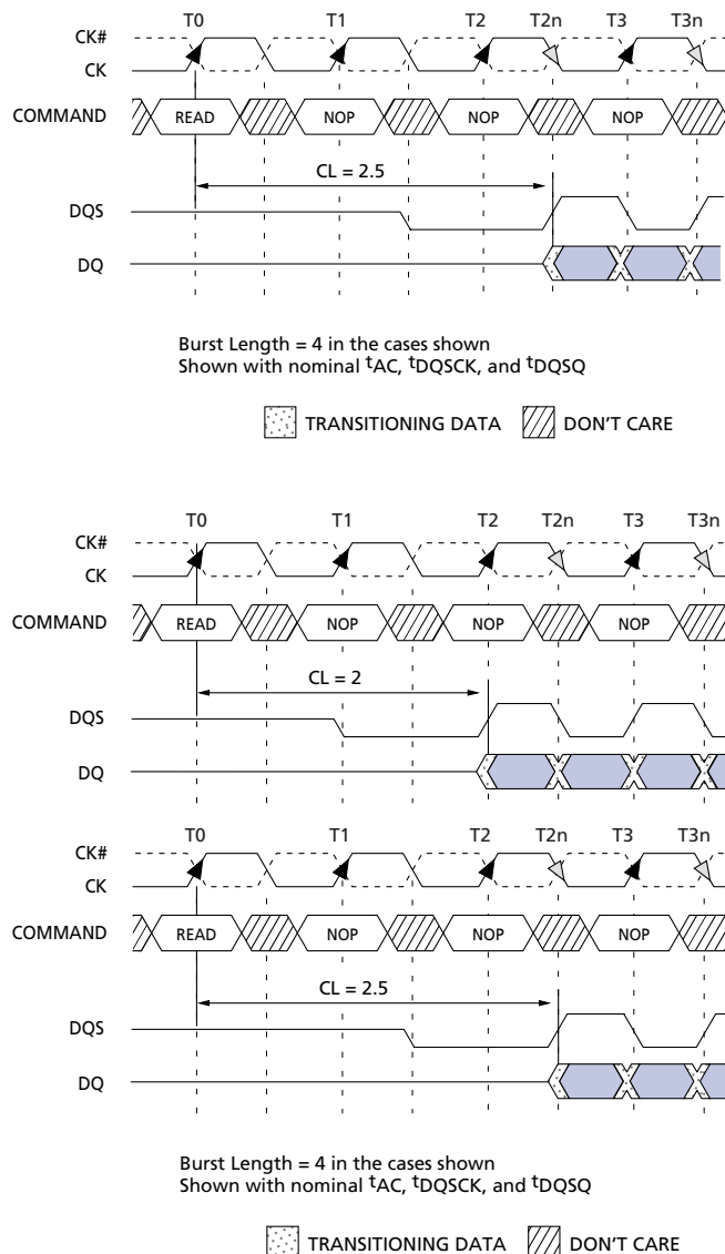
Figure 5: CAS Latency Diagram
