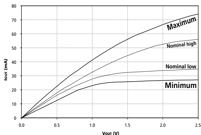
Figure 10: Reduced Output Drive Curve Pull-Down Characteristics
