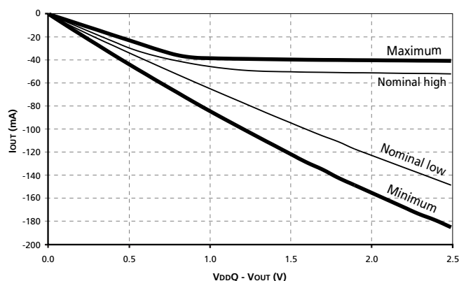
Figure 9: Normal Output Drive Curve Pull-Up Characteristics
