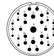
36-9 14 #16(A-G,Z-f) 14 #12(H-N,S-Y) 2 #8(O,R) 1 #4(P)
