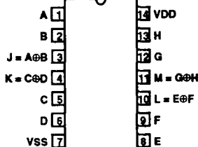
CD4077BMS TOP VIEW
