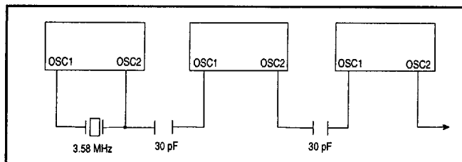
Figure 8 Common Crystal Connection
