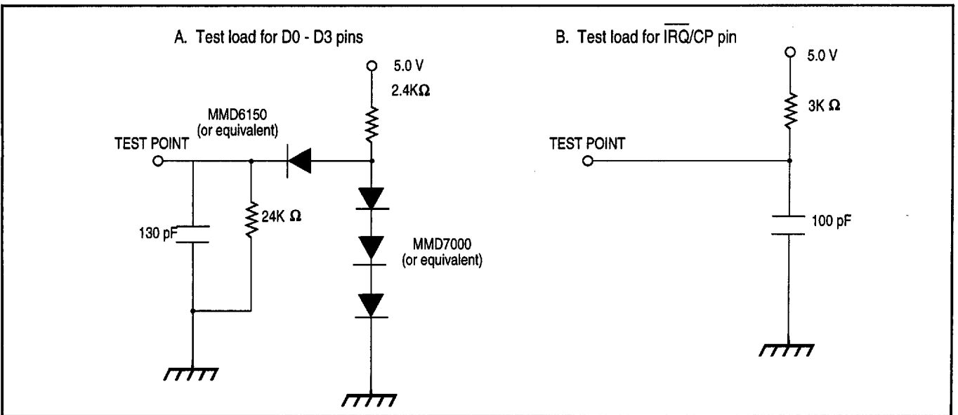
Figure 12 Test Loads
