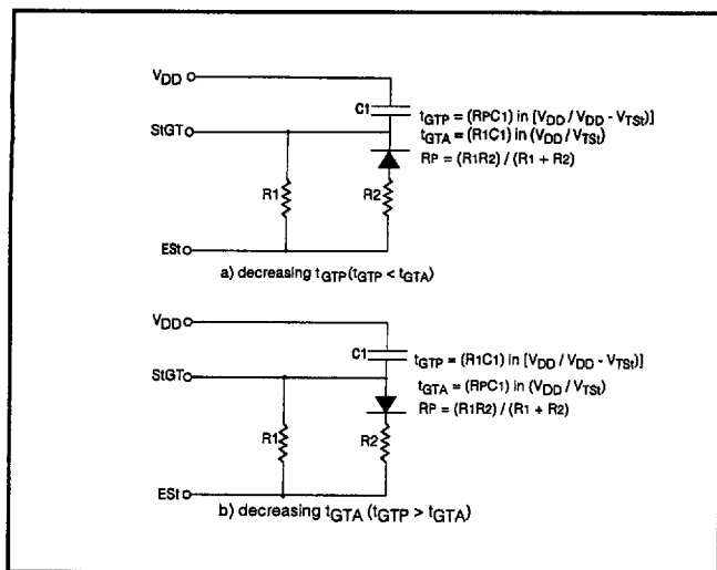
Figure 6 Guard Time Adjustment
