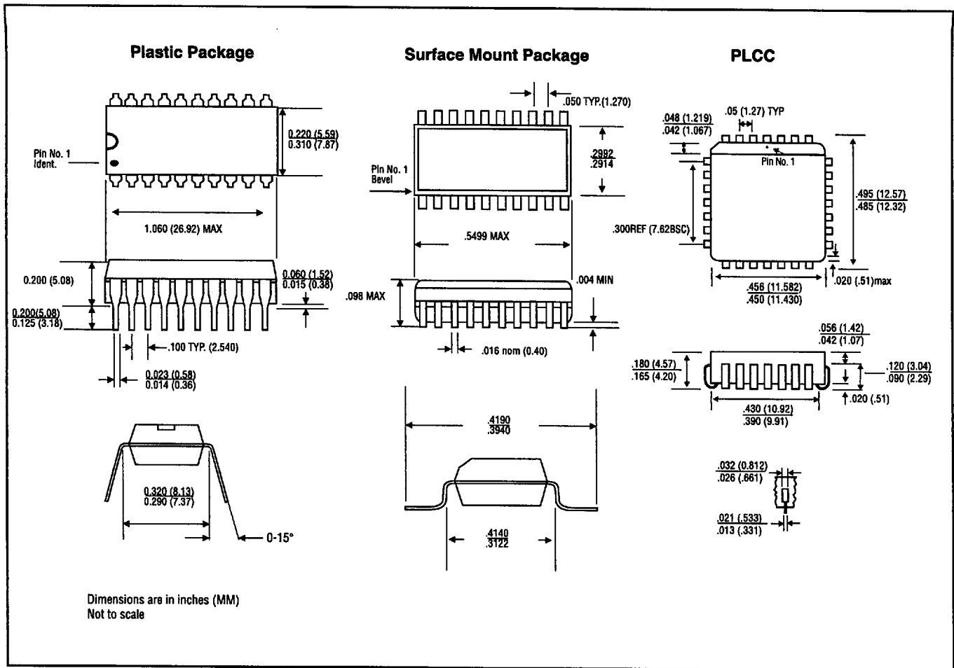
Figure 9 Package Dimensions
