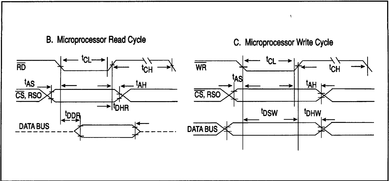
Figure 11 Timing Diagrams (continued)
