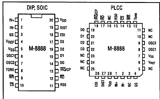
Figure 1 Pin Connections
