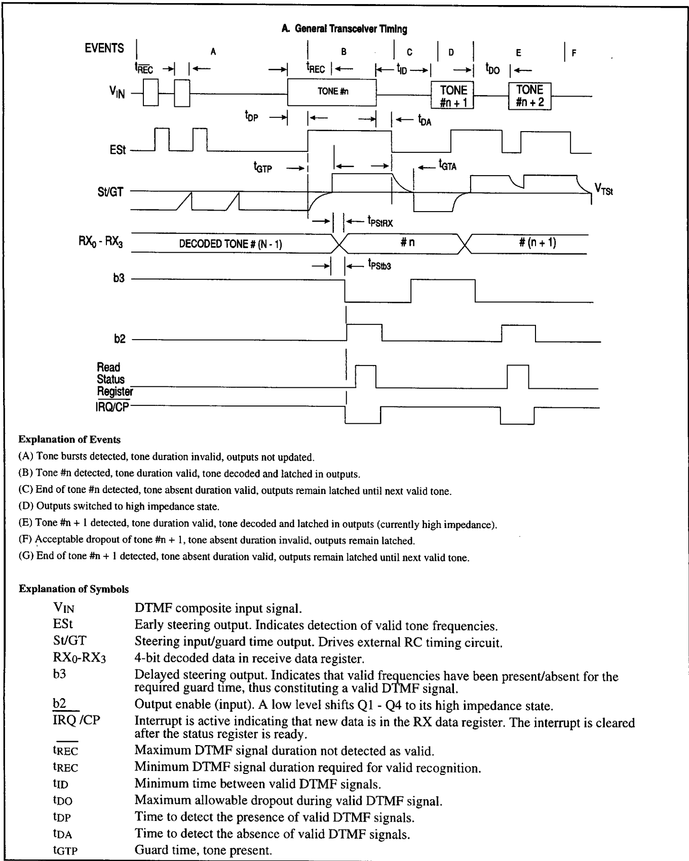
Figure 11 Timing Diagrams
