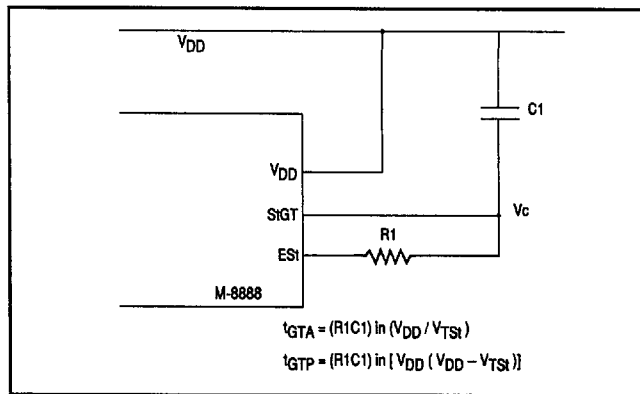
Figure 5 Basic Steering Circuit
