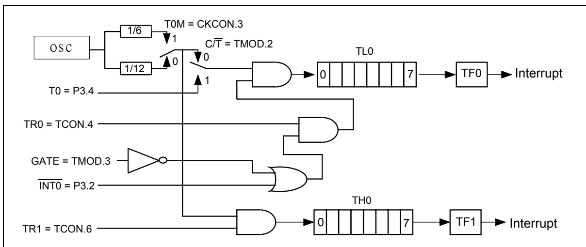
Timer/Counter 0 Mode 3
