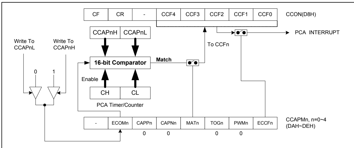
PCA 16-bit Timer Comparator Mode
