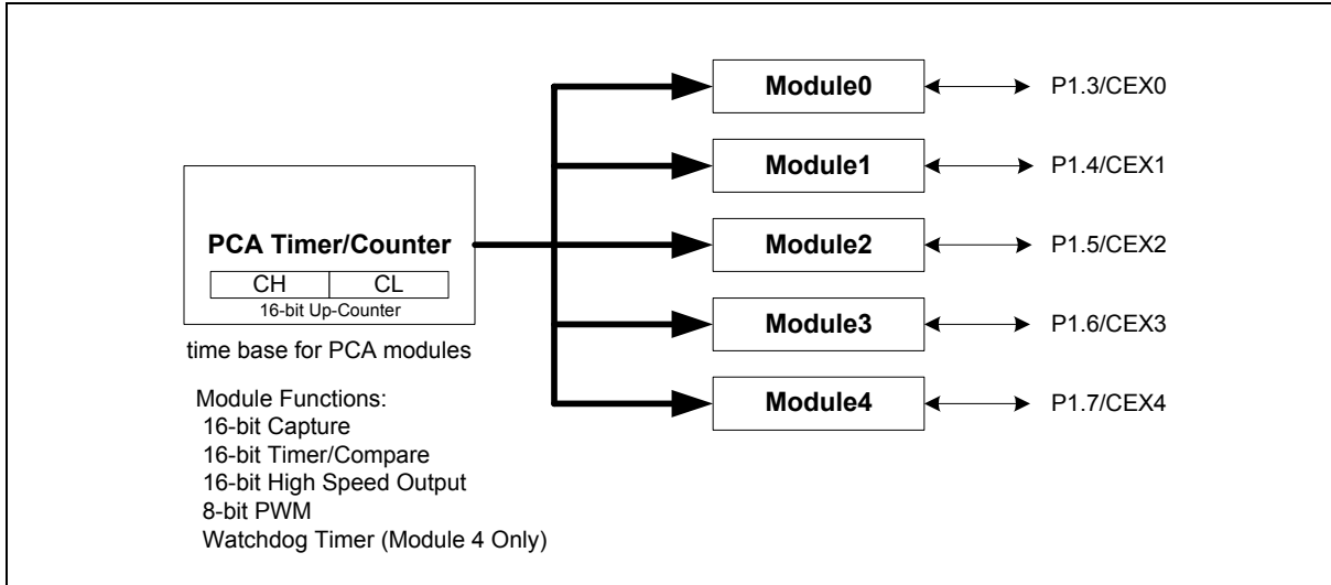
Programmable Counter Array (PCA)
