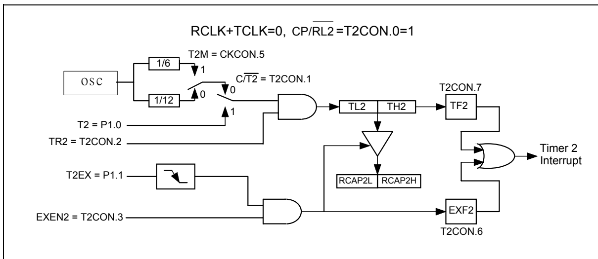
16-Bit Capture Mode
