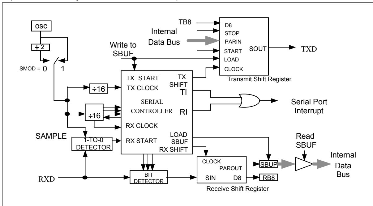
Serial Port Mode 2
