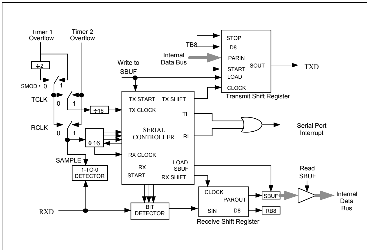
Serial Port Mode 3
