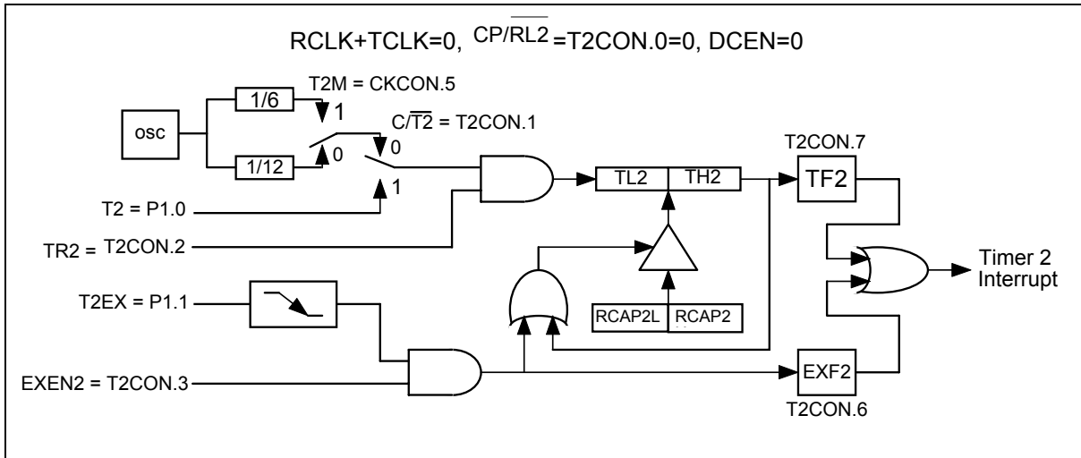
16-Bit Auto-reload Mode, Counting Up
