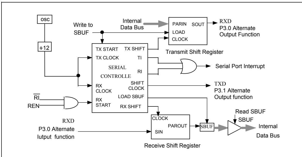
Serial Port Mode 0
