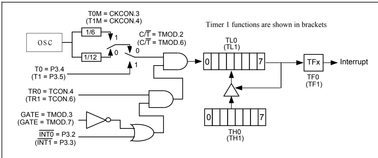
Timer/Counter Mode 2
