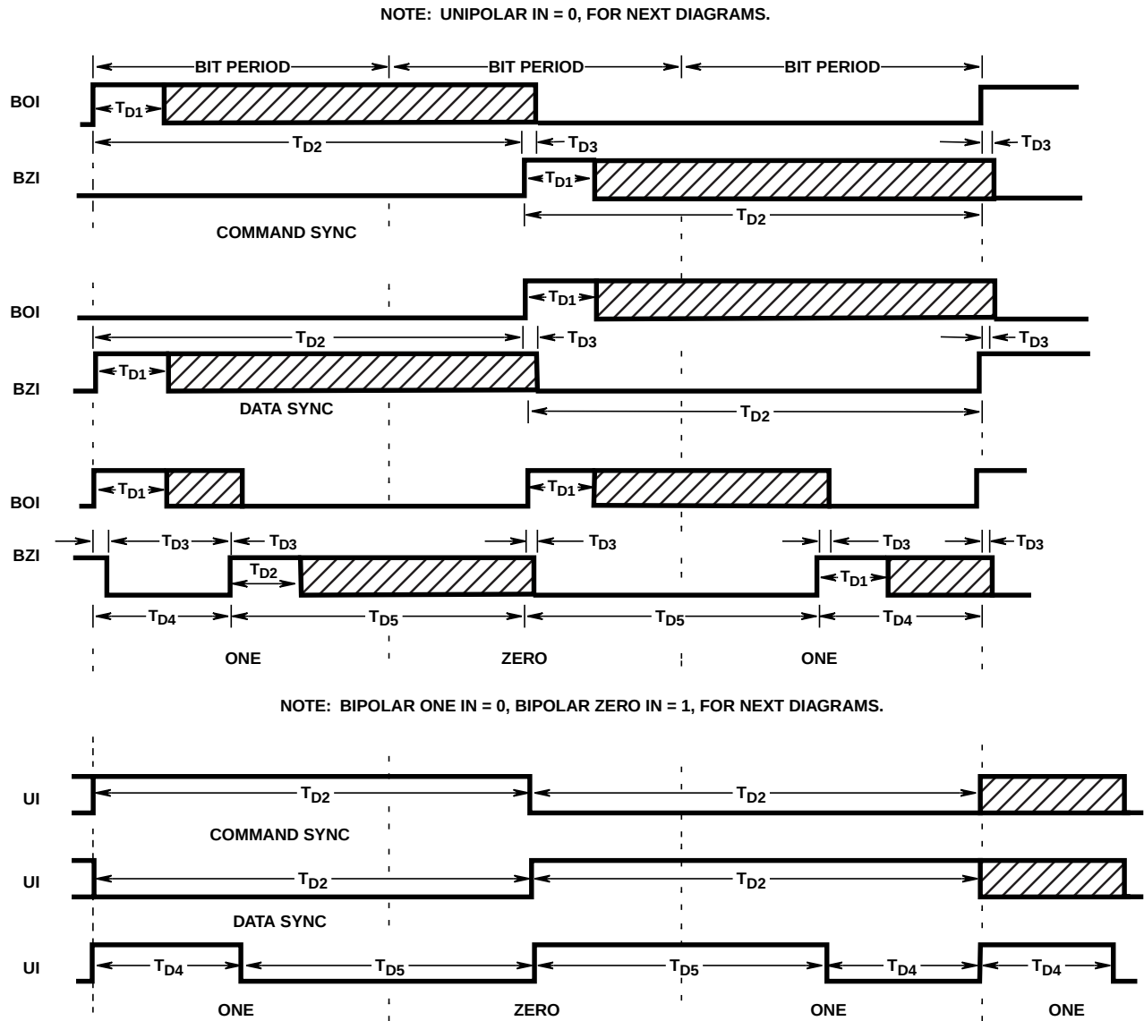
FIGURE 11. DECODER TIMING
