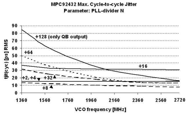
Figure 8. MPC92432 Cycle-to-Cycle Jitter
