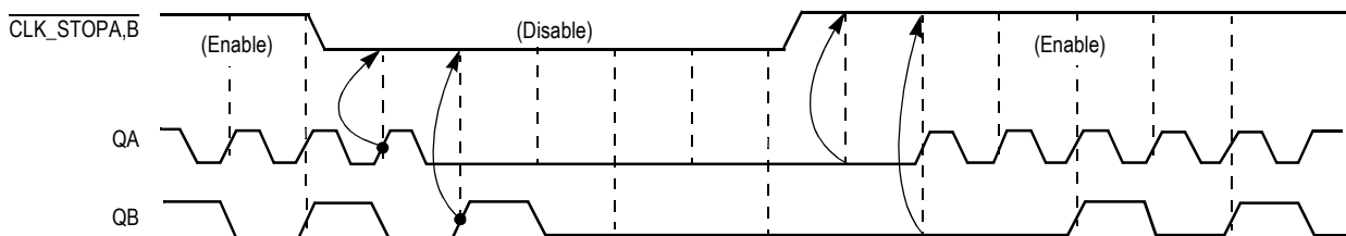
Figure 6. Clock Stop Timing for NB = 1 ( f_{QA} = 2 f_{QB} )
