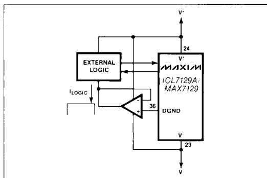
Figure 11. DGND Buffer
