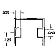
RFP-40-XXCAP (TOP CONDUCTOR)
