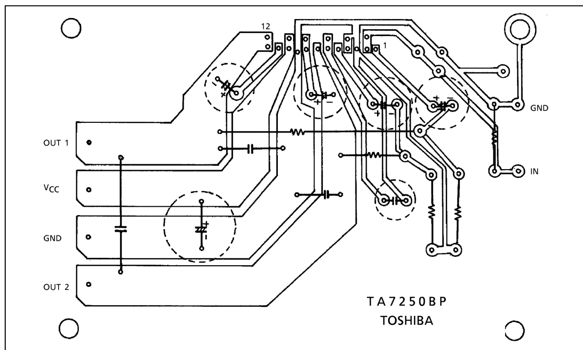
(Under view)
