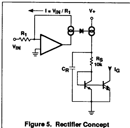
Figure 5. Rectifier Concept
