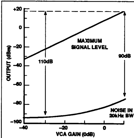
Figure 12. Dynamic Range of NE570
