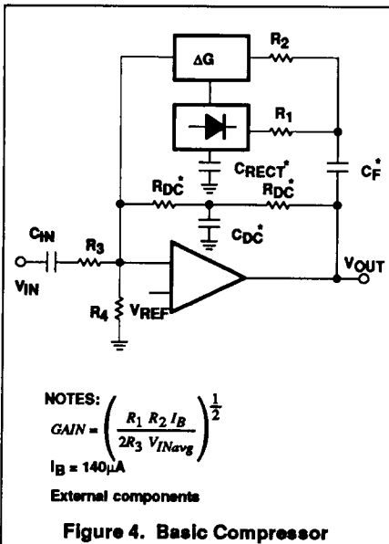
Figure 4. Basic Compressor
