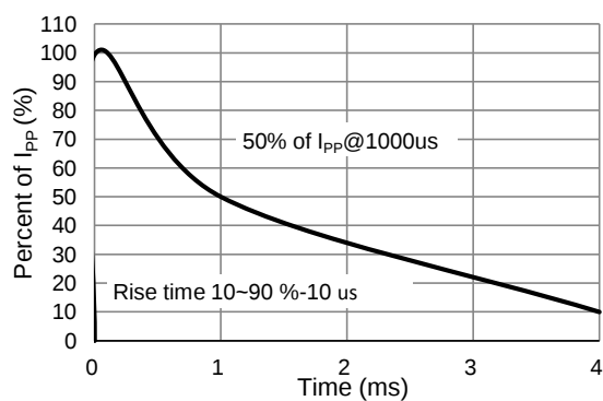
Fig.3 10/1000us Pulse Waveform
