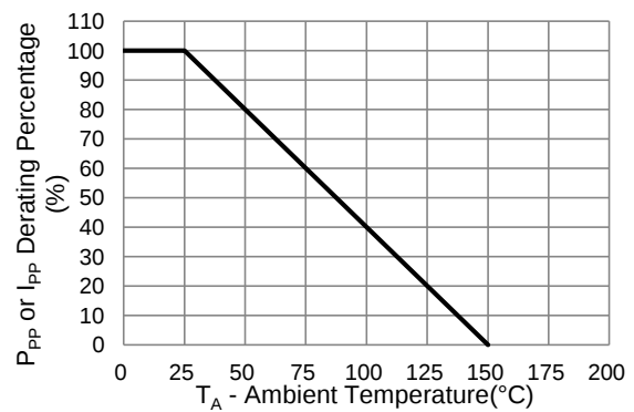
Fig.2 Derating Curve
