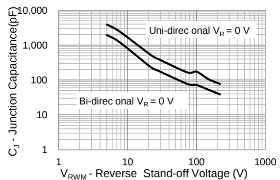
Fig.4 Typical Capacitance
