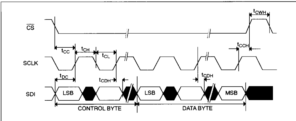
Figure 12. 29C310 Serial Data Input Timing Diagram
