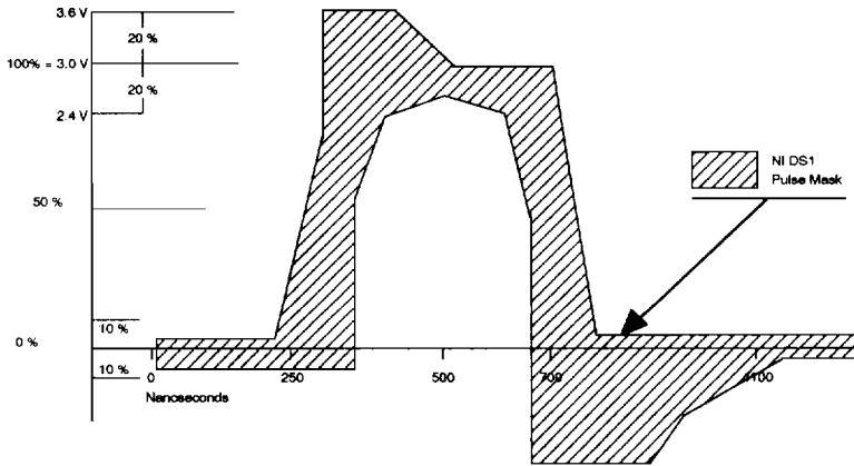
Figure 4. 1.544 MHz T1 Pulse Mask.
