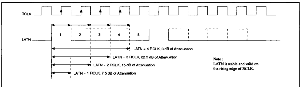
Figure 7. LATN Pulse Width Encoding
