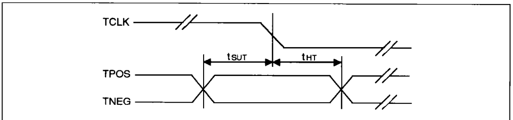
Figure 3. 29C310 Transmit Clock Timing
