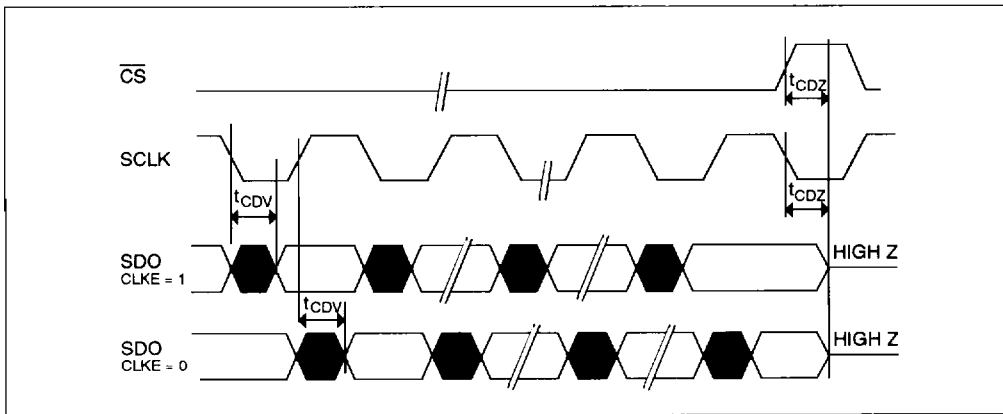
Figure 13. 29C310 Serial Data Output Timing Diagram
