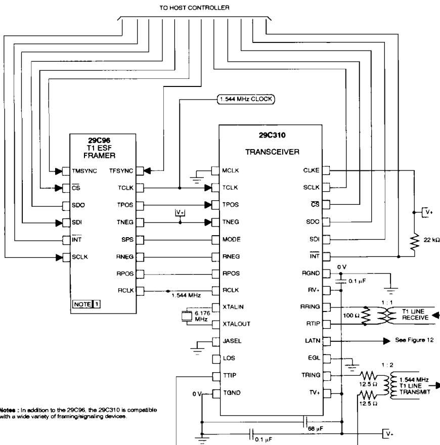
Figure 10. Typical 29C310 Host Mode T1/CSU Application
