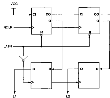
Figure 9. Typical LATN Decoding Circuit.
