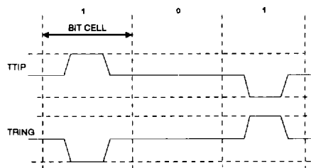
Figure 5. 50 % Ami Coding Diagram.
