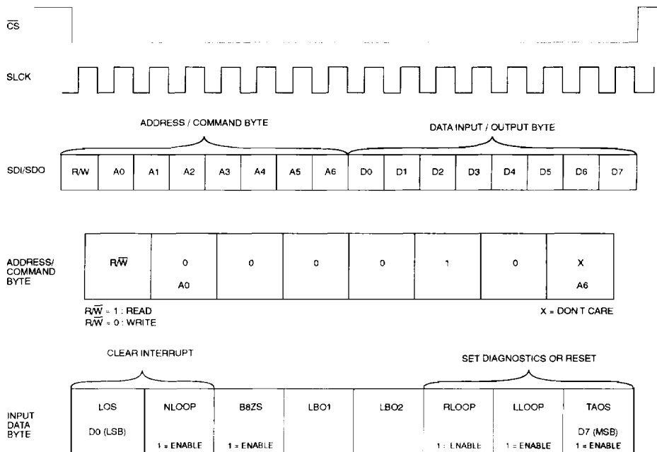
Figure 8. 29C310 Serial Interface Data Structure
