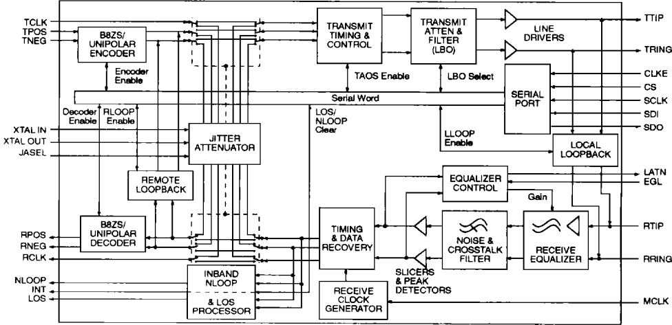
Figure 1. 29C310 Block Diagram
