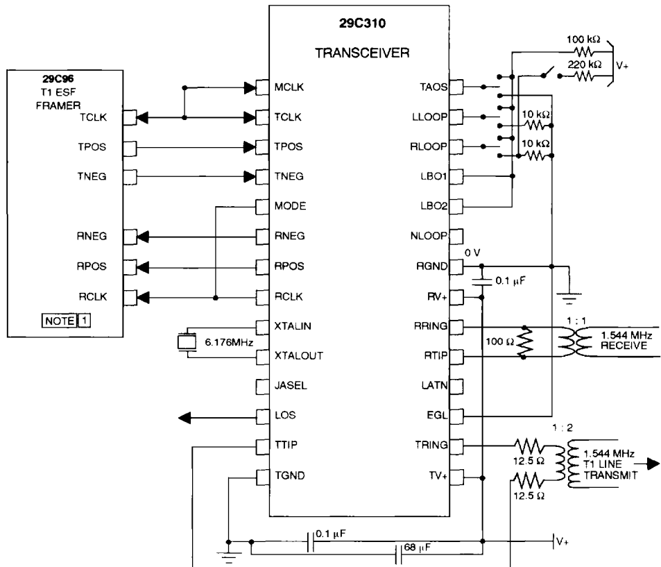
Figure 11. Typical 29C310 Hardware Mode Application.
