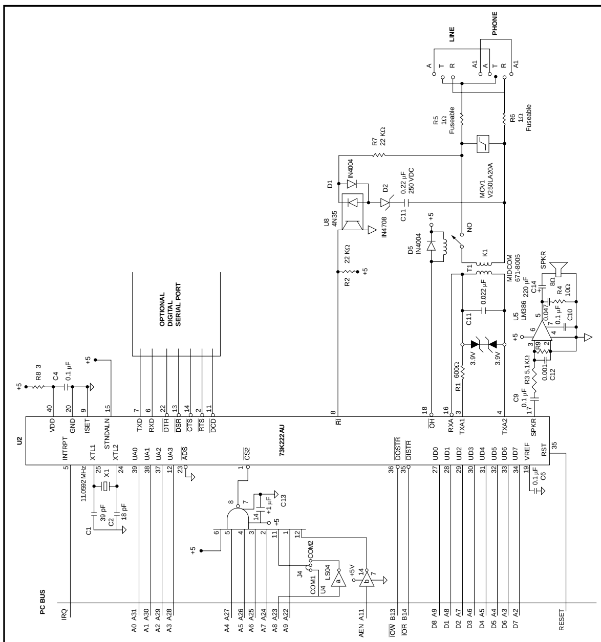
FIGURE 9: 73K222AU Typical Integral Application Single-Port Mode
