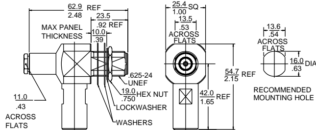
Type N Clamp Bulkhead Jack
