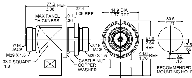
7-16 Jack to 7-16 Bulkhead Jack Adapter
