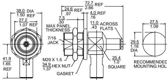
7-16 Clamp Bulkhead Jack
