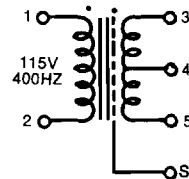
SCHMATIC "TS" (CENTER TAP)
