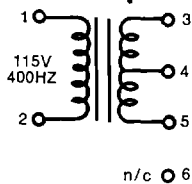
SCHMATIC "T" (CENTER TAP)
