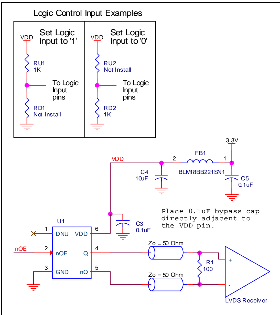
Figure 2. IDT8N4S272 Schematic Example
