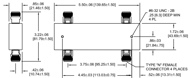
Andrew Type Number 245566 with N connector
