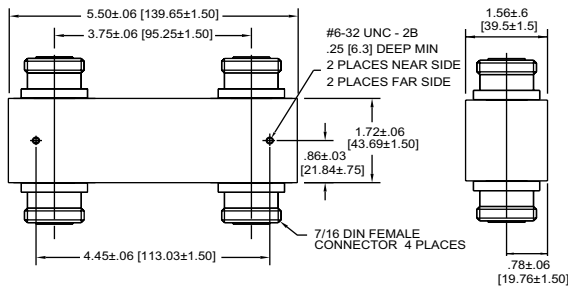
Andrew Type Number 245567 with 7-16 DIN connector
