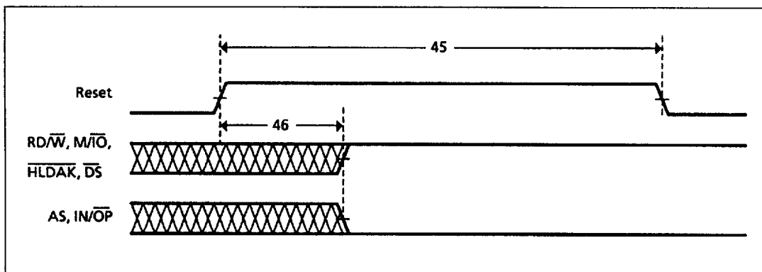
Figure 6: Reset Timing
