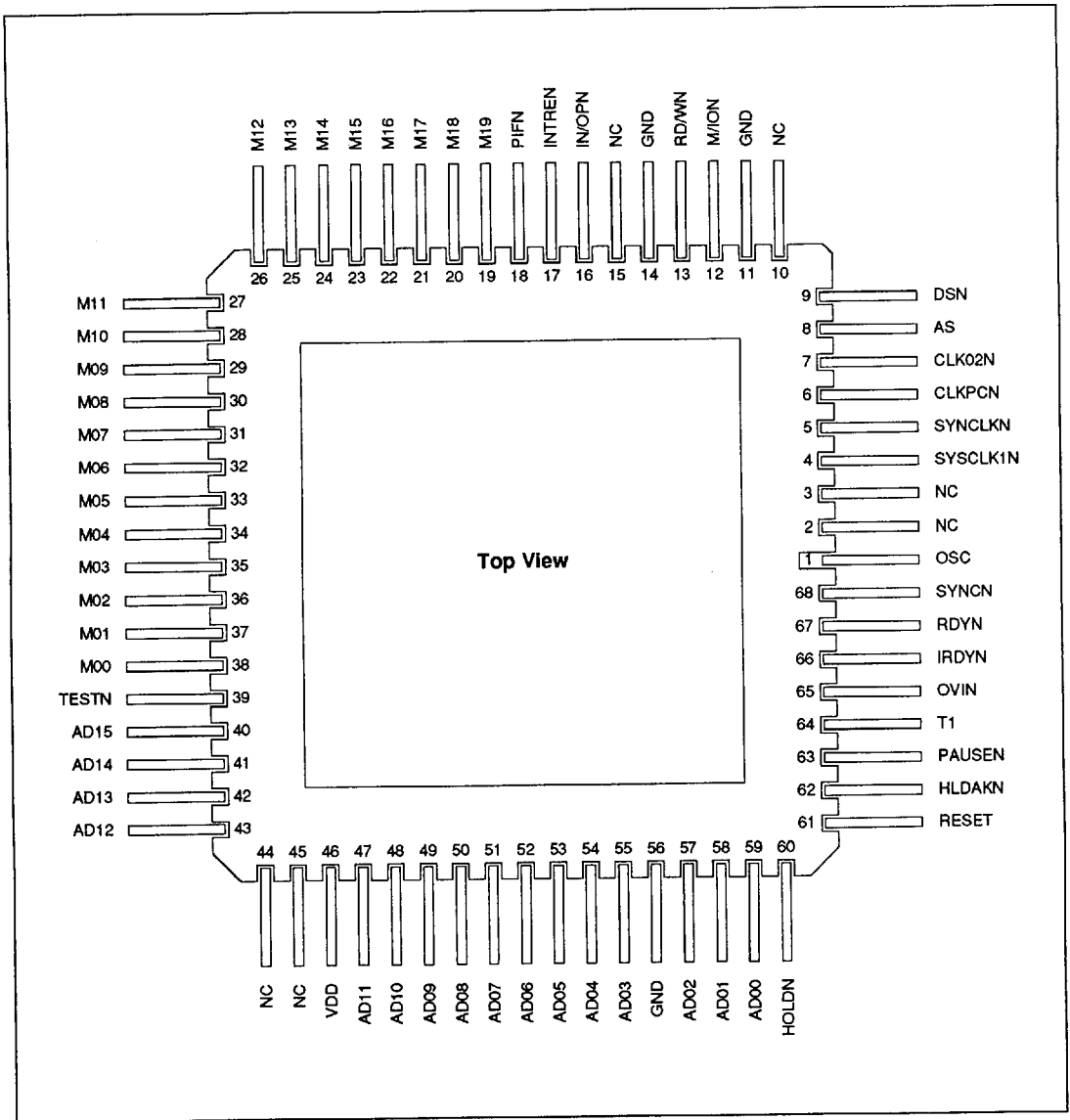
Figure 23b: Pin Assignments
