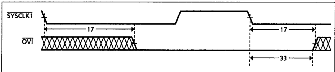
Figure 18: Fixed Point Overflow Timing
