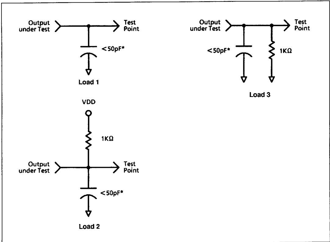
Figure 5: Test Loads
