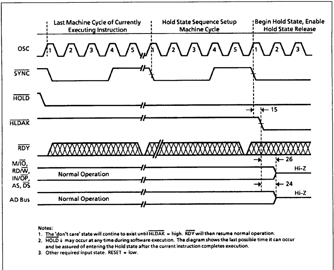
Figure 16: Hold State Generation Timing
