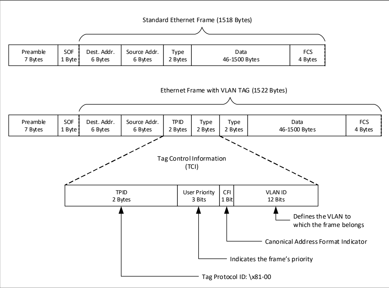
FIGURE 11-1: VLAN FRAME
