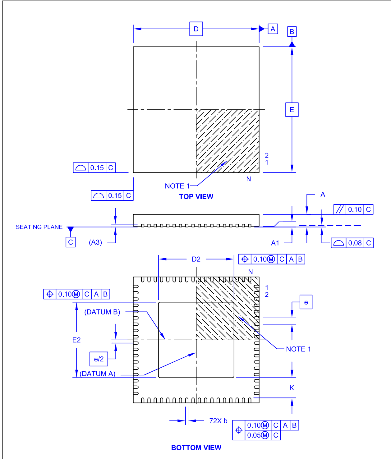
FIGURE 21-1: 72-QFN PACKAGE
