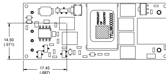
Figure 21. T_{ref} Temperature Measurement Location for V_o=12V .
