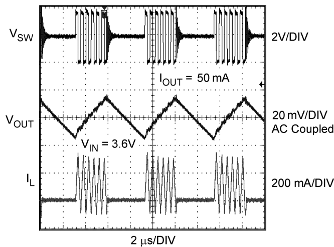
FIGURE 7. PFM Operation
