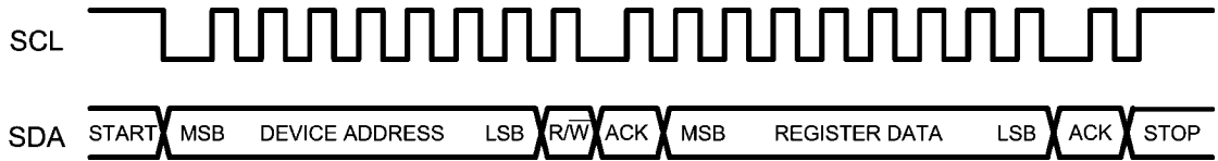
FIGURE 4. I 2 C Write Cycle
